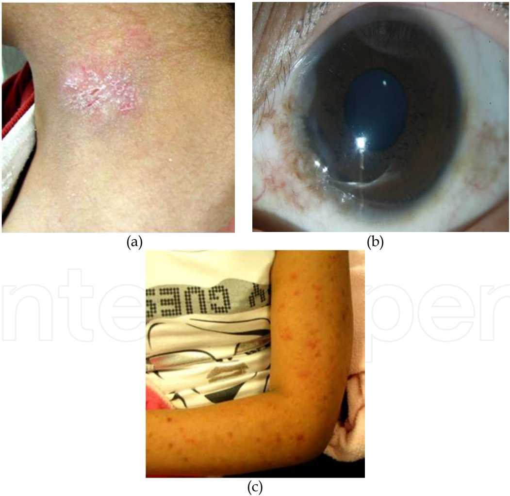
Fig. 2. Skin co-morbidities in patients with AC. Clinical pictures of Atopic Dermatitis in neck (a); Actinic Conjunctivitis (b); and Actinic Prurigo in forearm (c)
