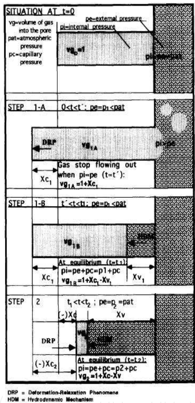
Fig. 2. Schematic representation of vacuum impregnation of an ideal pore. Deformation-relaxation phenomena and hydrodynamic mechanism occurring during vacuum period ( t_1 ) and relaxation time ( t_2 ) (from Fito et al., 1996).
