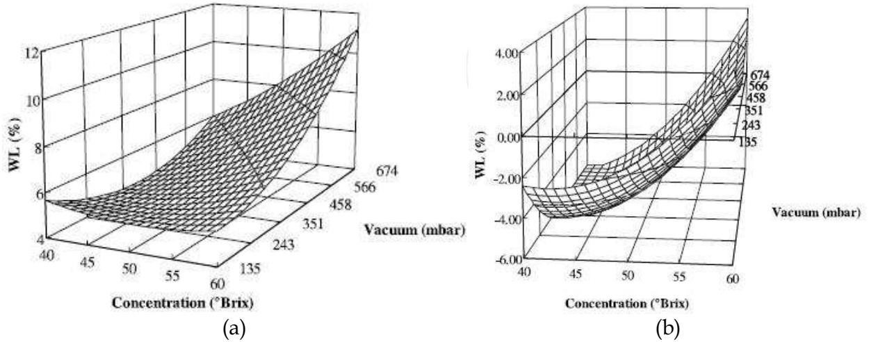
Fig. 8. Effects of vacuum pressure and osmotic solution concentration on water loss of mango and apples samples (from Mujica-Paz et al., 2003).
