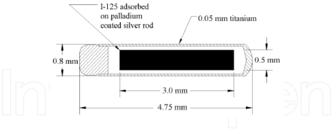
Fig. 10. Assembly of laser welded 125 I seed
