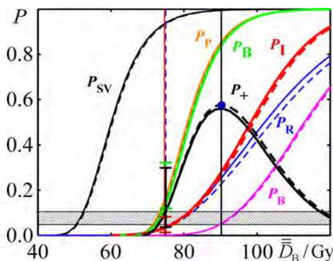
Fig. 6. The dose-response curves that are derived from the radiobiological evaluation of the dose distributions are plotted using \bar{\bar{D}} on the dose axis. The horizontal crossed bar indicates the 5-10% response probability region. The solid and dashed vertical lines indicate the dose levels of the dose distributions with and without setup correction, respectively. The vertical error bars indicate the confidence intervals of the corresponding dose-response curves due to the uncertainties of the radiobiological parameters. The solid lines correspond to the dose distribution with setup correction, whereas the dashed lines correspond to the dose distribution without setup correction.
