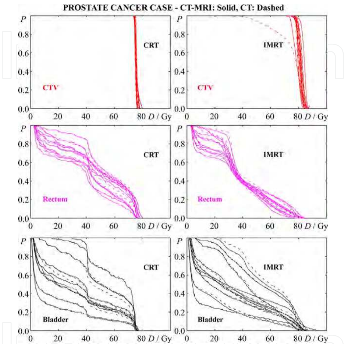
Fig. 2. The dose volume histograms (DVHs) of the CTV, rectum and bladder are presented in the upper, middle and lower diagrams, respectively for the CRT (left) and IMRT (right) treatment plans, which were optimized based on the CT and fused CT-MRI images, separately.
