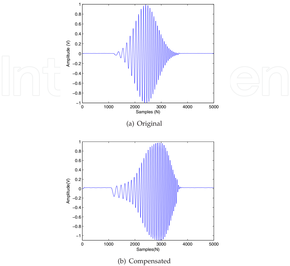
Fig. 5. Transmitted gaussian chirps signals [40-200 kHz].
