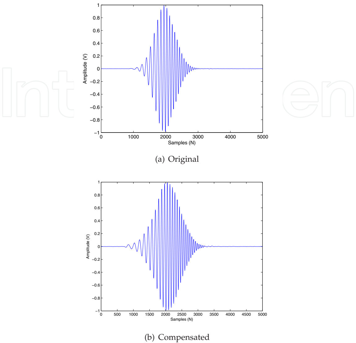
Fig. 6. Received gaussian chirps signals [40-200 kHz].
