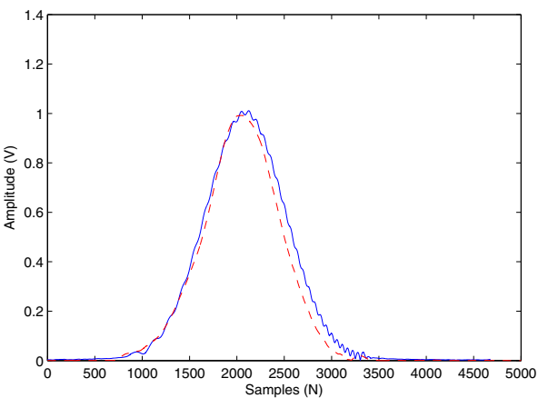
(b) The Hilbert Tranform of the original transmitted signal (solid curve) and the signal received following compensated transmission (dashed curve).
