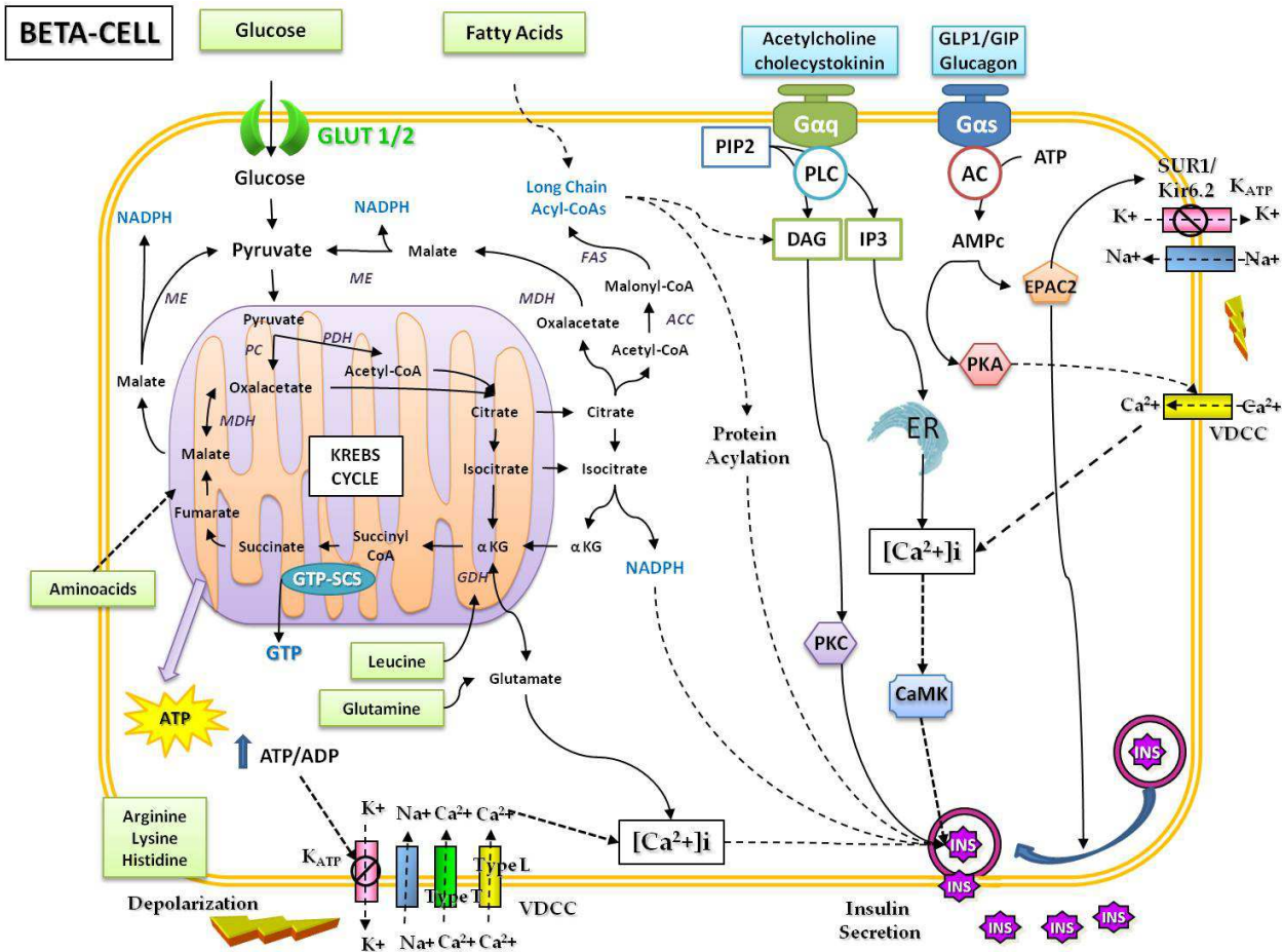
Fig. 2. Regulation of glucose-stimulated insulin secretion by nutrients, hormones and neurotransmitters. Glucose-stimulated insulin secretion may be modulated by several mechanisms. Glucose metabolism increase ATP/ADP ratio and closes ATP-sensitive pottasium channels ( K_{ATP} ), depolarizing the membrane, opening voltage-dependent calcium channels (VDCC), and thus increasing intracellular calcium ( [Ca^{2+}]_i ). Glucose metabolism by the Krebs Cycle also renders a series of metabolic coupling factors that may initiate and sustain insulin secretion. These metabolic coupling factors participate in mitochondrial shuttles, involving NADPH, pyruvate, malate, citrate, isocitrate, acyl-CoAs, and glutamate. Signaling pathways that contribute to maintaining or increasing glucose-stimulated insulin secretion include PKA and PKC. Glucagon, glucagon-Like peptide 1 (GLP-1), and glucose-dependent insulintropic peptide (GIP) act through PKA pathway, while acetylcholine and cholecystikinin act through the PKC pathway. Fatty acids may contribute to insulin secretion through the PKC pathway through formation of diacylglycerol (DAG) or through protein acylation. Aminoacids may stimulate insulin release by increasing ATP production from the Krebs Cycle, by membrane depolarization, or by participating in intracellular calcium increase. ( \alpha KG : alpha-ketoglutarate, ACC: Acetyl CoA Carboxylase, FAS: Fatty Acid Synthase, GDH: Glutamate Dehydrogenase, GTP-SCS: GTP-Succinyl CoA Synthetase, ER: endoplasmic Reticulum, ME: Malic enzyme, MDH: Malate Dehydrogenase, PC: Pyruvate Carboxylase, PHD: Pyruvate Dehydrogenase, PIP2: Phosphatidyl Inositol Biphosphate, IP3: inositol 1,4,5-trisphosphate ).
