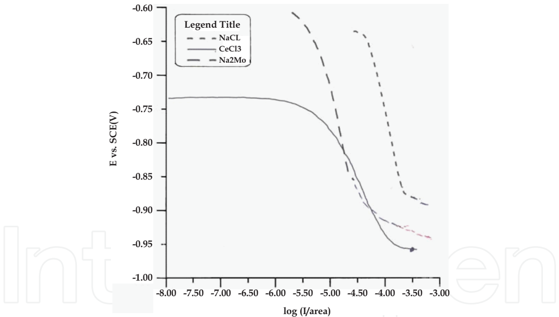
Fig. 11. A cathodic polarization curve of temper T4 of the alloy in 3.5 wt% NaCl + 1000 ppm CeCl 3 in deaerated condition (Zaki, 2009)
