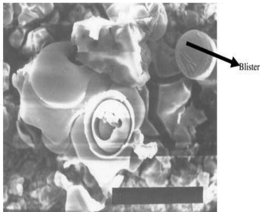
Fig. 15. Broken oxide layer forming blisters (mothballs)
