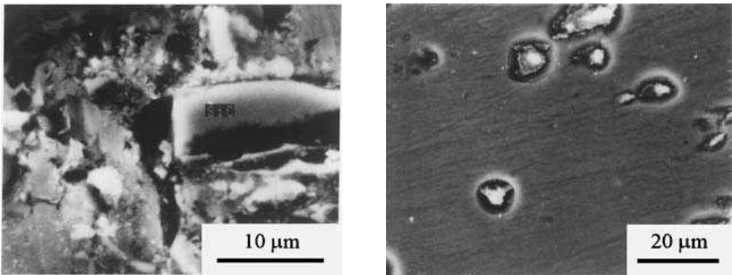
Fig. 5. Scanning electron micrographs of pits on interfaces of (a) SiCp-2024 Al matrix, and (b) inclusions-2024 Al matrix (Feng et al., 1998)
