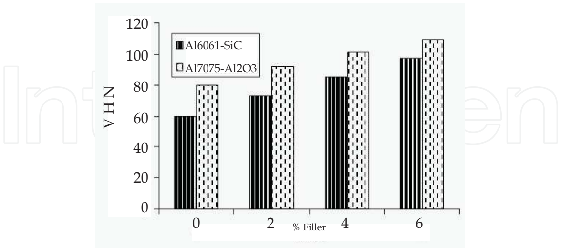
Fig. 1. Microhardness of Al6061-SiC and Al7075-Al2O3 composites (Vaeeresh et al., 2010)
