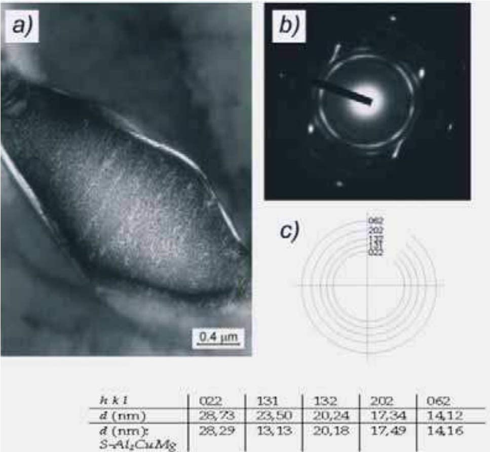
Fig. 7. Microstructure of the AlCu4Ni2Mg alloy: a) precipitates of S-Al 2 CuMg phase, b) electron diffraction pattern obtained from the precipitate, c) solution of the diffraction pattern
