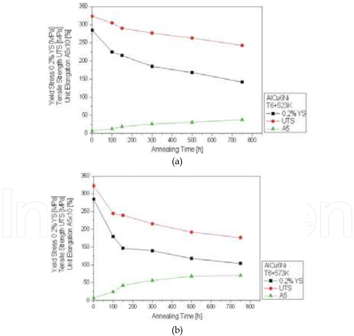
Fig. 21. Ultimate tensile strength, 0.2% offset yield strength and elongation A 5 for AlCu6Ni alloy as a function of annealing time at the temperature of a) 523K and b) 573 K
