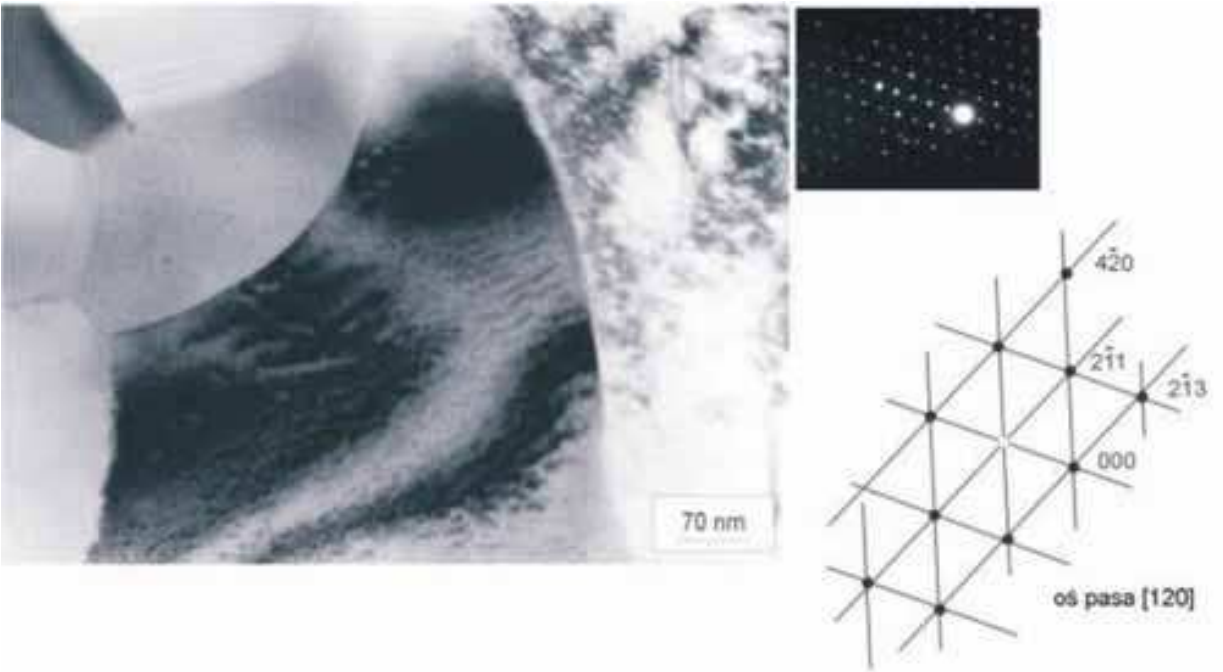
Fig. 8. Microstructure of the AlCu6Ni alloy: particle of \alpha -Al 2 CuMg phase
