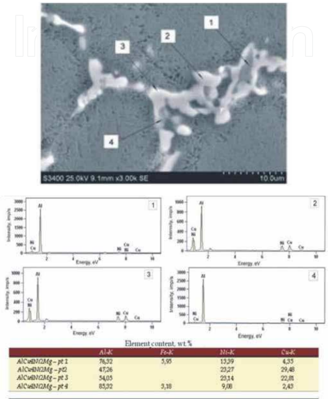
Fig. 5. AlCu 4 Ni 2 Mg alloy – EDS analysis of the areas 1–4
