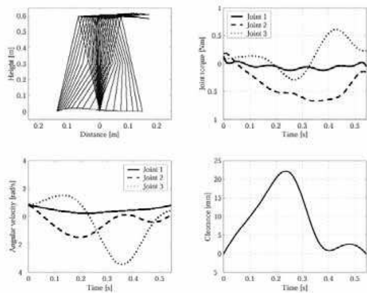
Fig.12. The result of using inequality constraint at intermediate time ( \delta = 20[\text{mm}] , S = 0.150[\text{m}] , T = 0.55[\text{s}] ) (Hase T. & Huang, Q., 2005).
