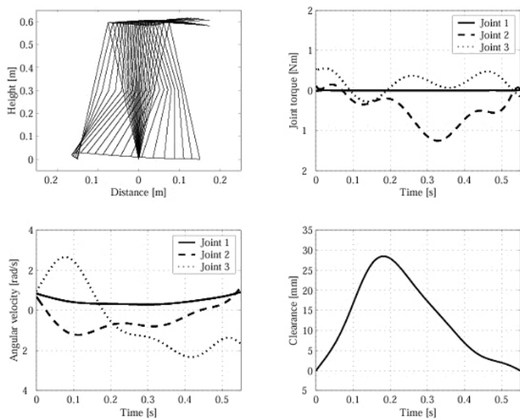
Fig.13. The result of using inequality constraint at intermediate time ( u_1 = 0 , \delta = 20[\text{mm}] , S = 0.150[\text{m}] , T = 0.55[\text{s}] ) (Hase T. & Huang, Q., 2005).
