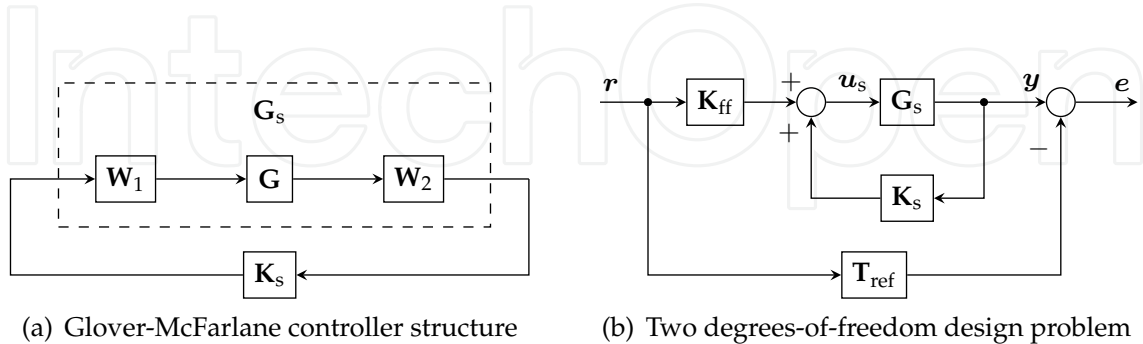
Fig. 5. Loop-shaping controllers
