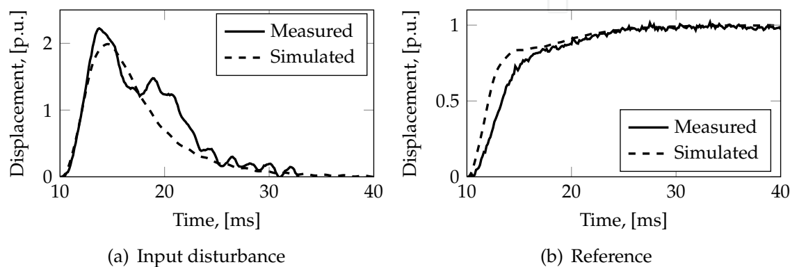
Fig. 10. Step responses.
