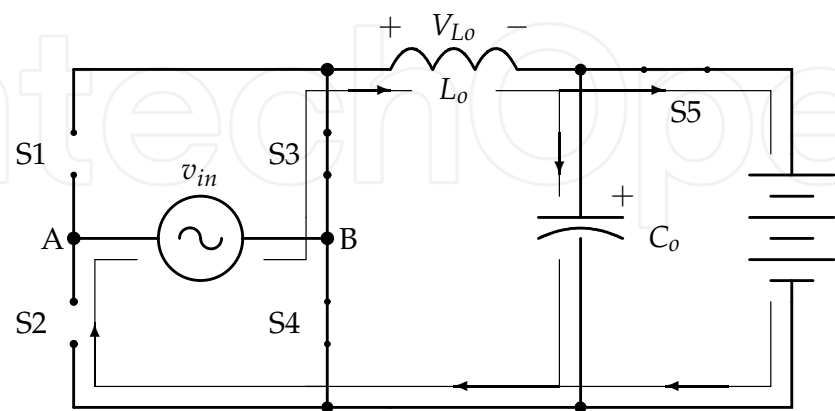
(c) Discharging of inductor through S2 & S3
