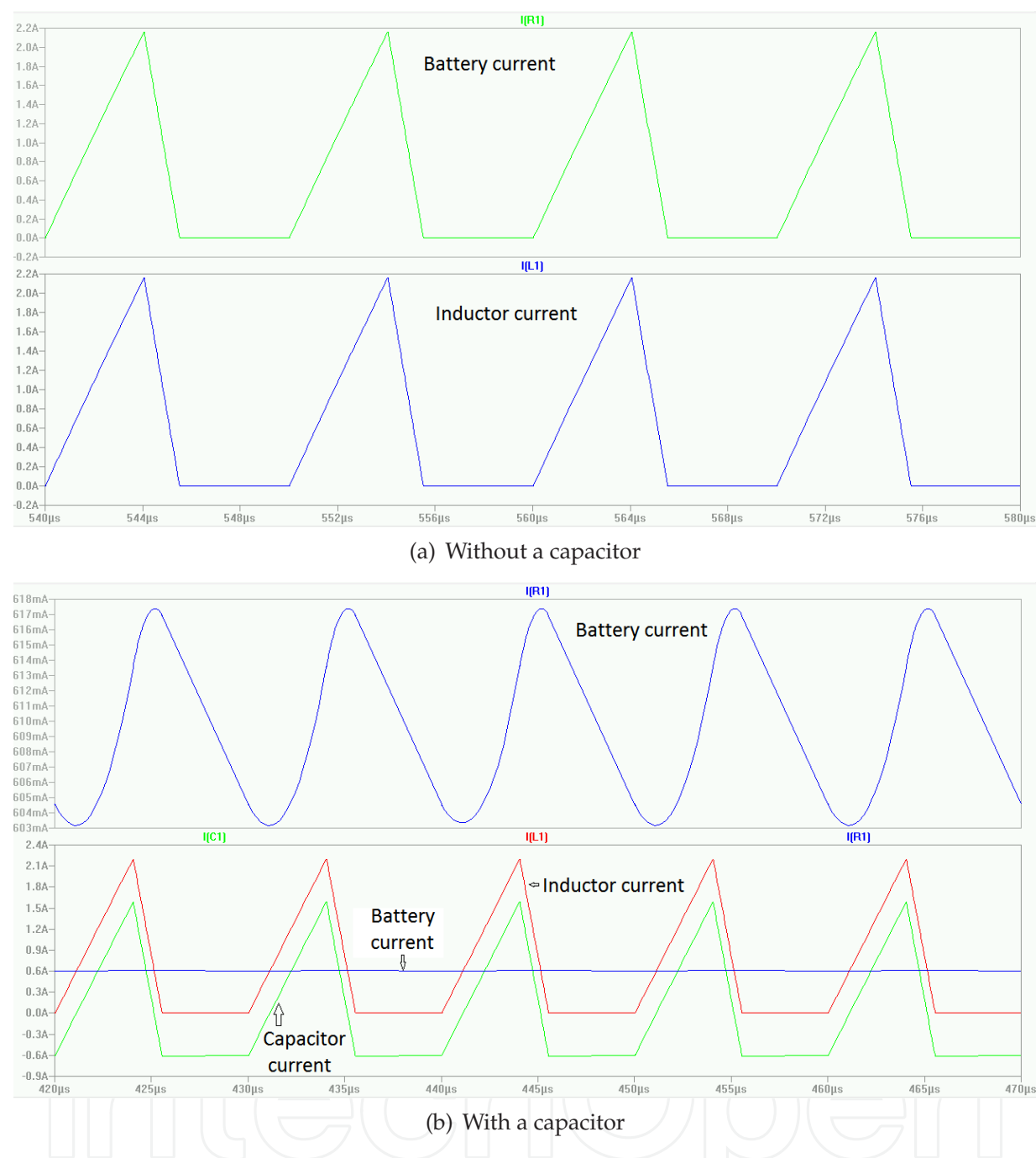
Fig. 10. The importance of capacitor placed in parallel with the battery.
