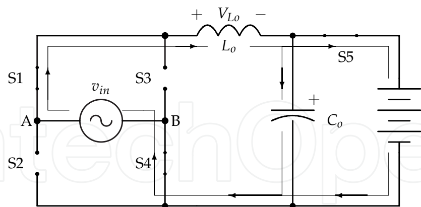
(a) Charging of inductor
