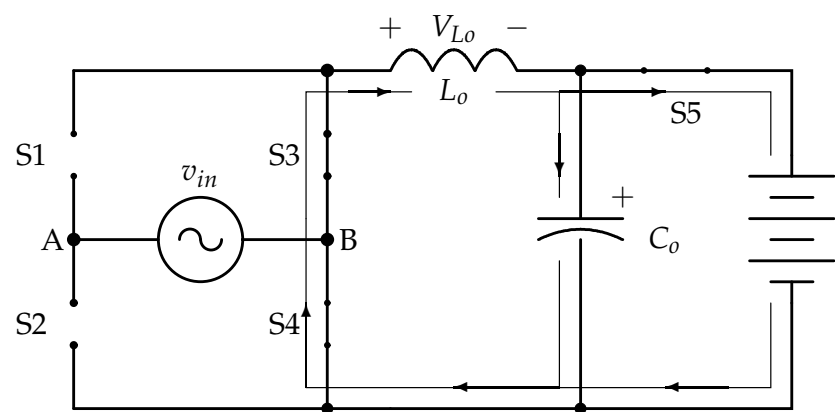
(b) Discharging of inductor through S3 & S4
