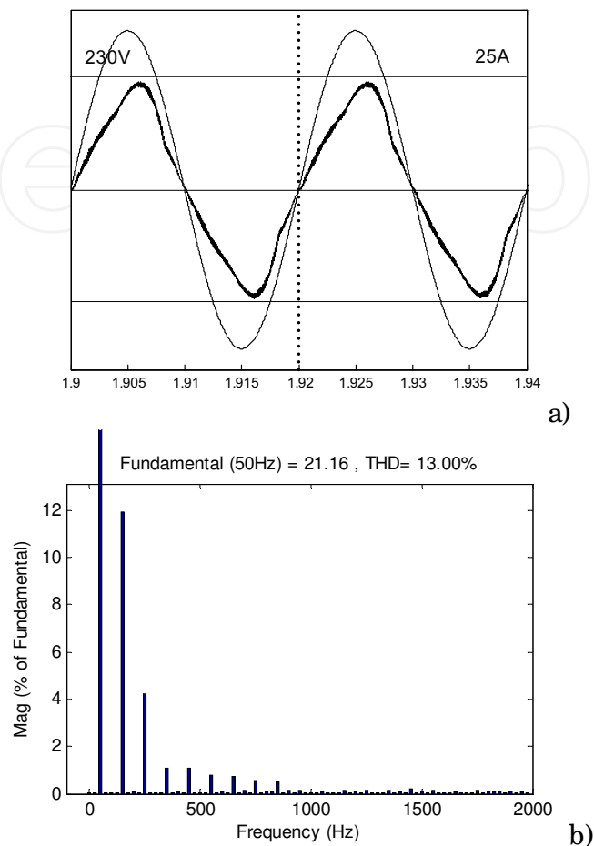
Fig. 23. a) Waveforms of grid voltage and \mu G current; b) \mu G current harmonics and \text{THD}_i=13\%
