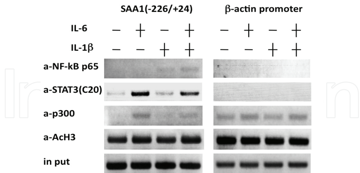
Fig. 4. Chromatin immunoprecipitation assays demonstrate recruitment pattern of STAT3, NF- \kappa B p65, and p300 on the SAA1 promoter (-226/+24) from HepG2 cells treated with IL-6 (10 ng/ml) and/or IL-1 \beta (0.1 ng/ml) for 30 min. Anti-AcH3 antibody was used as a positive control for this assay
