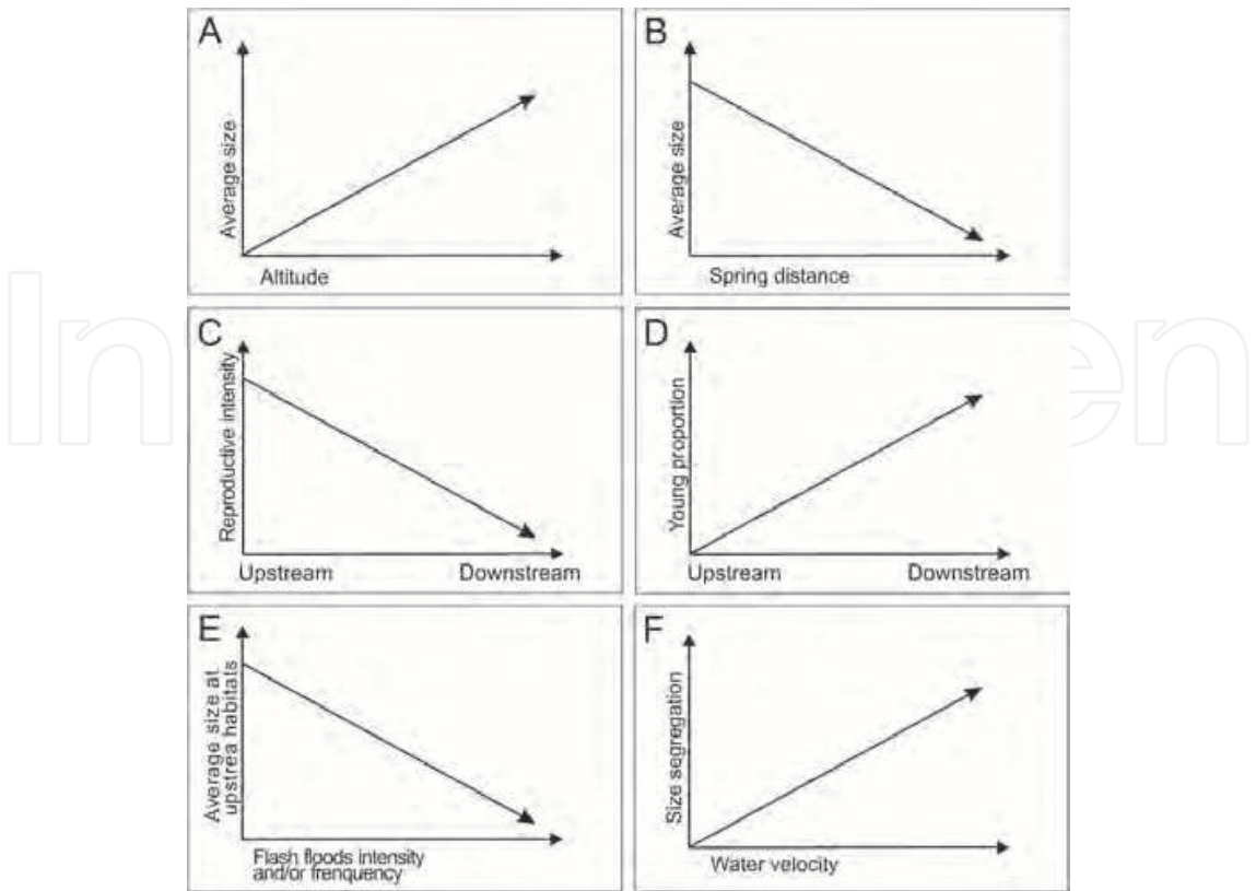
Fig. 5. Hypotheses of patterns and main drivers of the ontogenetic migration. A. Average size of individuals within a population increases towards higher altitude; B. Average size of individuals within a population decreases with spring distance; C. Population’s reproductive intensity decreases along the longitudinal gradient from upstream to downstream; D. Proportion of young individuals increases along the longitudinal gradient from upstream to downstream; E. Average size of the individuals within a population decreases with higher flash flood intensity and/or frequency; F. Size segregation becomes more evident as water velocity increases (Illustration by Igor Kintopp).
