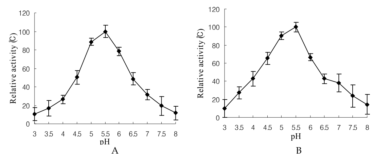
Fig. 4. Effects of pH on activity (A) and stability (B) of purified Bacillus megaterium KLP-98 protease (Fu et al., 2008).
