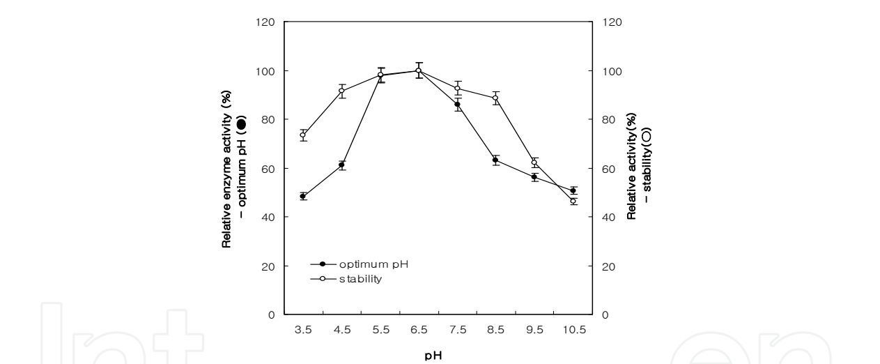
Fig. 5. Effects of pH on activity (A) and stability (B) of purified Aspergillus oryzae LK-101 protease (Hwang et al., 2010).
