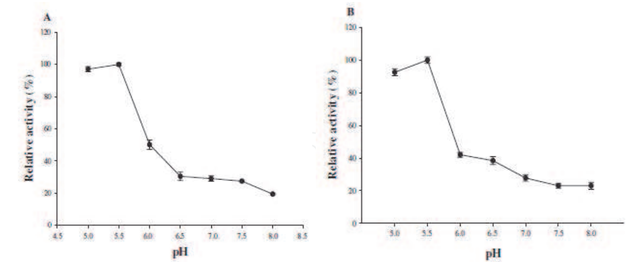
Fig. 3. Effects of pH on activity (A) and stability (B) of purified Bacillus subtilis JM3 protease (W.J. Kim and S.M. Kim, 2005).
