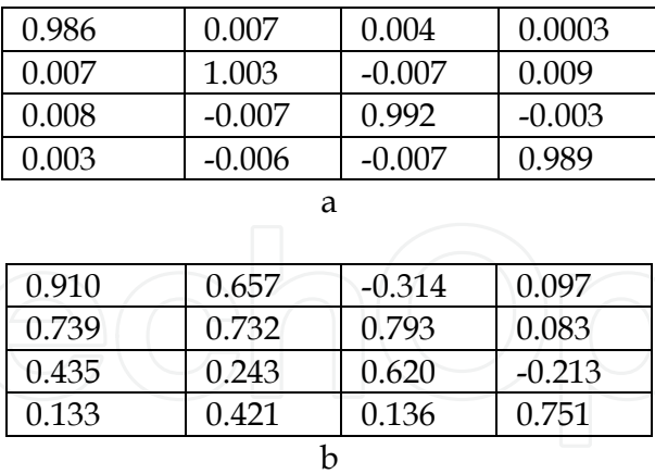
Fig. 6. Mueller matrix data for transmitted polarized laser beam (a) no sample (air) and (b) for scattering turbid sample.
