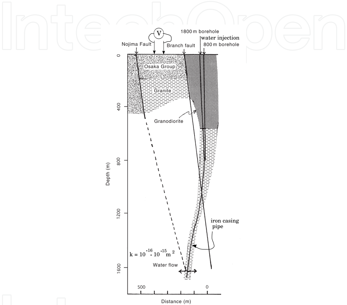
Fig. 6. Measurement of the permeability of the Nojima fault (modified from Murakami et al. (2001)). The water injection inside the borehole of 1800 m depth crosses the fault inducing an electrokinetic source at depth within the fault. The conduction current is conducted by the iron pipe up to the surface. The difference of potential V is measured by electrodes on the surface. The permeability is deduced from eq. 15
