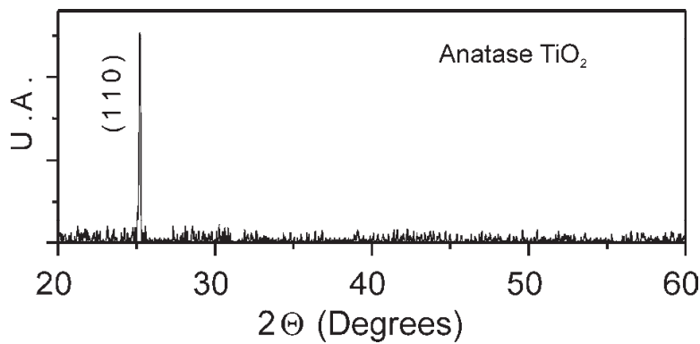
Fig. 5. XRD pattern of TiO 2 thin film, (take it on Shimadzu 6000 diffractometer with Cu-K α radiation (λ = 0.15418 nm) source).
