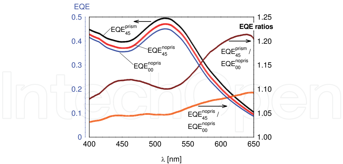
Fig. 25. Measured EQE for three simple configurations on a thin (3 \mu m) DSC. The three configurations correspond to normal incidence ( \theta=00^\circ ) without prism, oblique incidence ( \theta=45^\circ ) without prism and oblique incidence ( \theta=45^\circ ) with prism. The light spot is always wholly inside the active area (impinging power is constant). The enhancement ratios are retrieved normalizing the last two curves to the first one.
