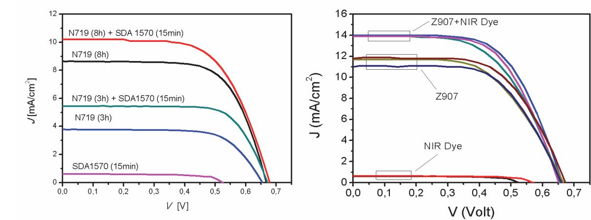
Fig. 16. J-V curves for N719-SDA (left) and Z907-SDA (right) co-sensitized systems. The lowest curve is due to the SDA sensitizer alone (labeled NIR in the right plot). It can be seen that the contribution of SDA is very small when compared to the N719 or Z907 current generation, but it becomes very important when the ruthenium dye is already and partially attached to the surface.
