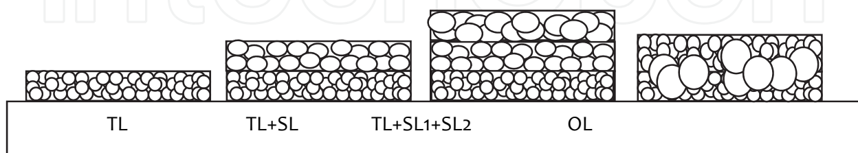
Fig. 18. From left to right hand: few micrometers nc- \text{TiO}_2 ( \sim 15\text{--}20\text{ nm} ); single scattering layer ( d \sim 100\text{ nm} ) on the previous; double scattering layer with upper one having d > 200\text{ nm} particle size; dispersion of small and large diameter \text{TiO}_2 particles. TL = Transparent layer, SL = Scattering Layer, OL = Opaque Layer.
