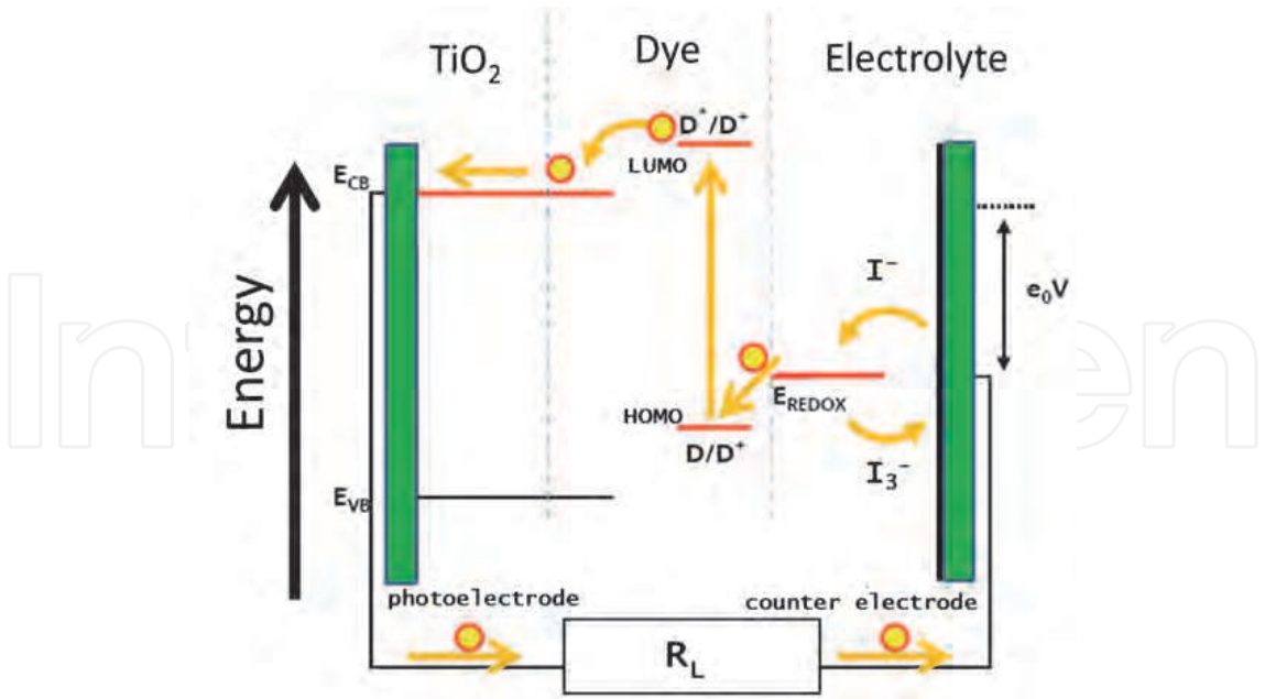
Fig. 3. DSC working principle: the absorption of a photon by a Dye molecule in its ground state D induce the transition to the excited state D^* . The injection of an e^- into the \text{TiO}_2 conduction band occurs, resulting in the Dye oxidation D^+ . The e^- diffuse into the \text{TiO}_2 reaching an external circuit and a load R_L where electrical power is produced. Successively it is reintroduced into the cell by the counter electrodes and regenerate the oxidized Dye D^+ utilizing a redox couple as mediator.
