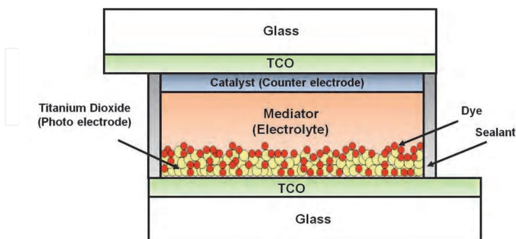
Fig. 1. Dye Solar Cell Structure. Basic cell's constituent are a transparent conductive substrate (TCO) coated glass and over it a nc-TiO 2 layer sensitized by a monolayer of adsorbed dye (photo-electrode), a red-ox mediator and, finally a catalyst (Pt) coated conductive substrate (counter-electrode).
