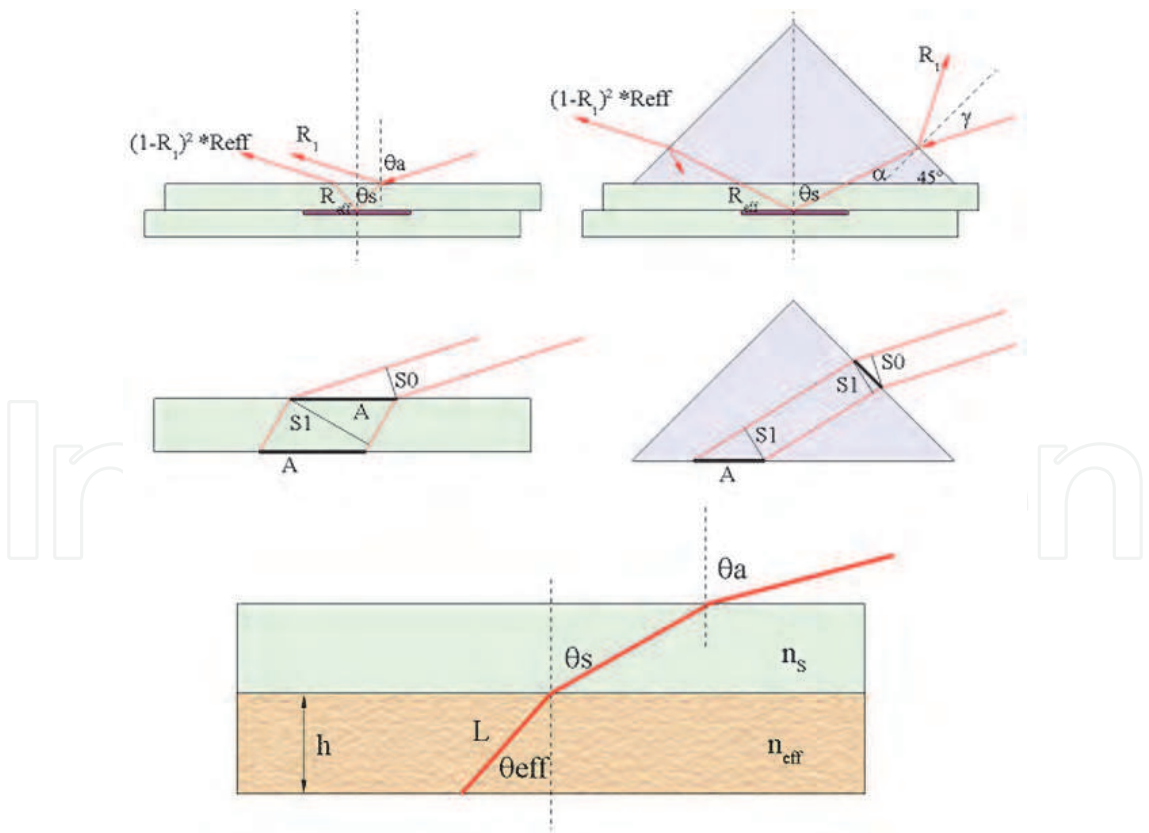
Fig. 26. Mechanism of the three main angular factors in the case of bare device and prism coupling. The considered effects are external reflectivity, projection of the active area and angular refractive path.
