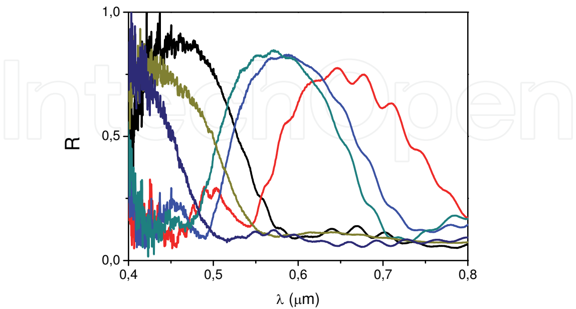
Fig. 22. Reflectance on nc-TiO 2 PEs containing SiO 2 /TiO 2 bi-layers measured by FTIR.
