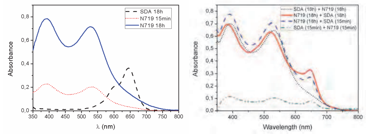
Fig. 15. Absorbance of 6 micrometers titania PEs in several dye adsorption configurations; (left) single dye TiO 2 attachment and (right) saturation conditions.
