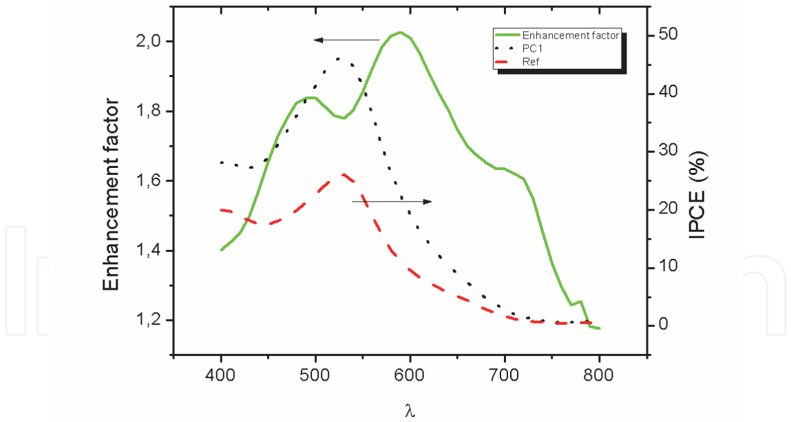
Fig. 23. IPCE enhancement factor calculated by the ratio between the PC integrated and the standard DSC.
