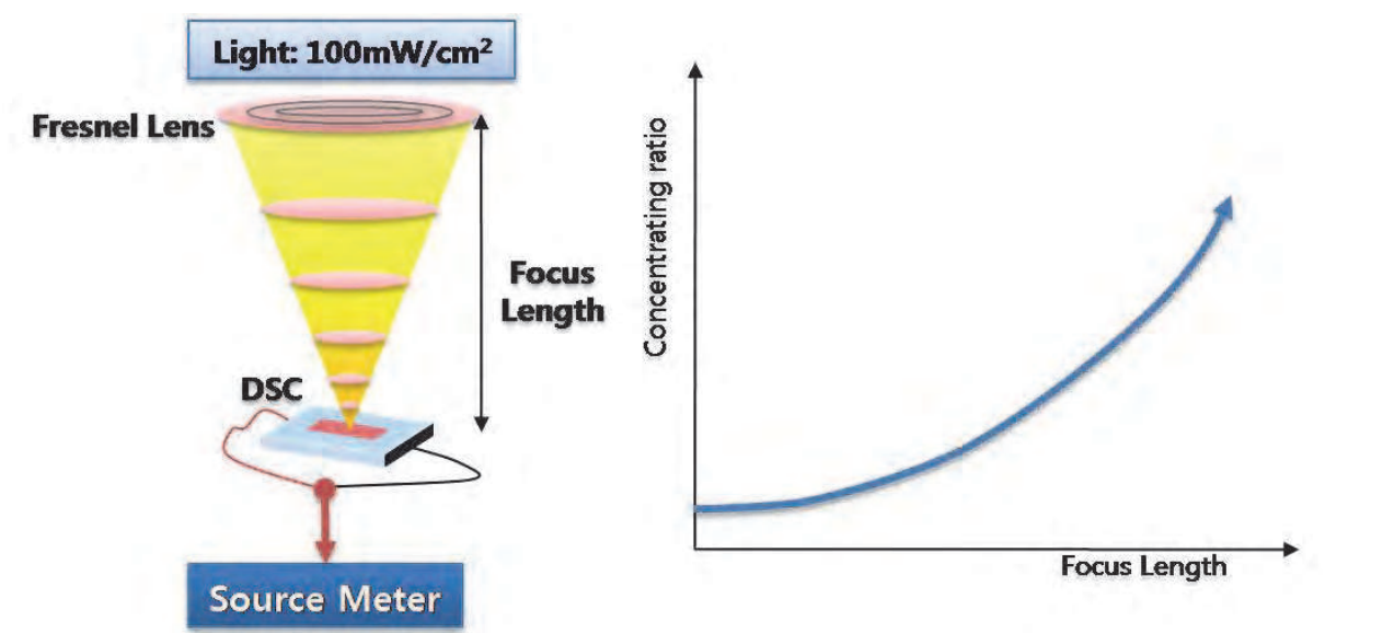
Fig. 24. Schematic of concentrating DSC
