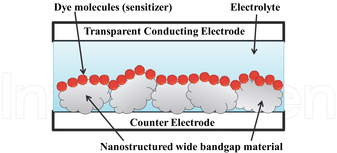
Fig. 2. Schematic of the structure of the dye sensitized solar cell.
