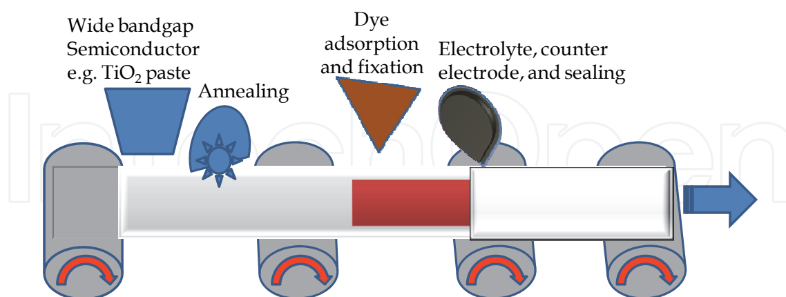
Fig. 23. Schematic of role-to-role manufacturing of flexible dye sensitized solar cells.
