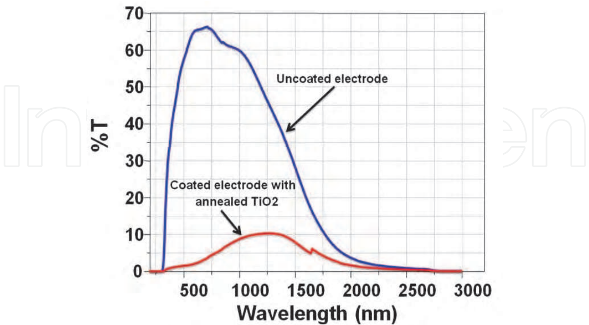
Fig. 3. Transmittance of conductive glass electrode before and after being coated with nanostructured \text{TiO}_2 layer.
