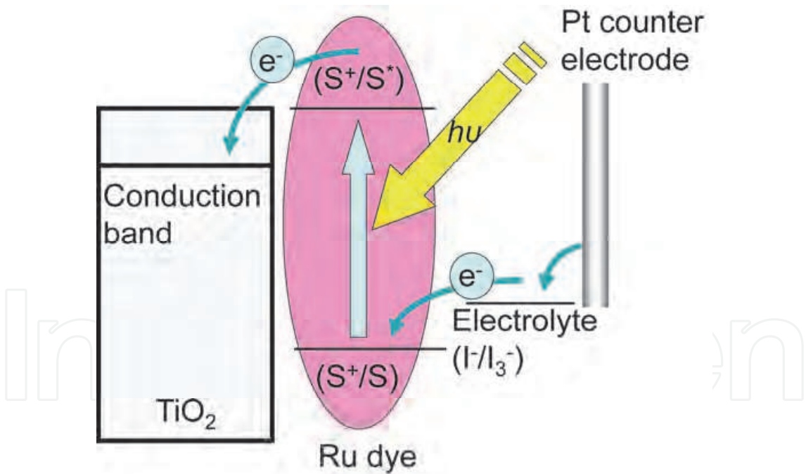
Fig. 6. Electron transfer in DSCs.
