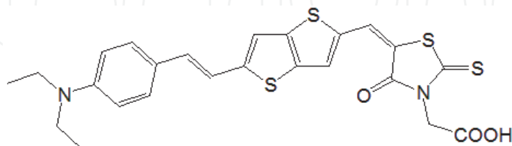
Fig. 29. Thienothiophene-thiophene-derived dye [25].
