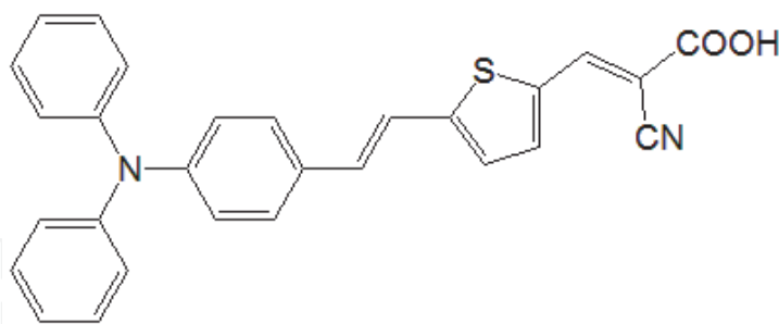
Fig. 26. Polyene-diphenylaniline dye [22].
