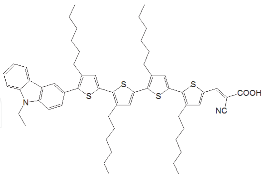
Fig. 32. Oligothiophene dye [29].
