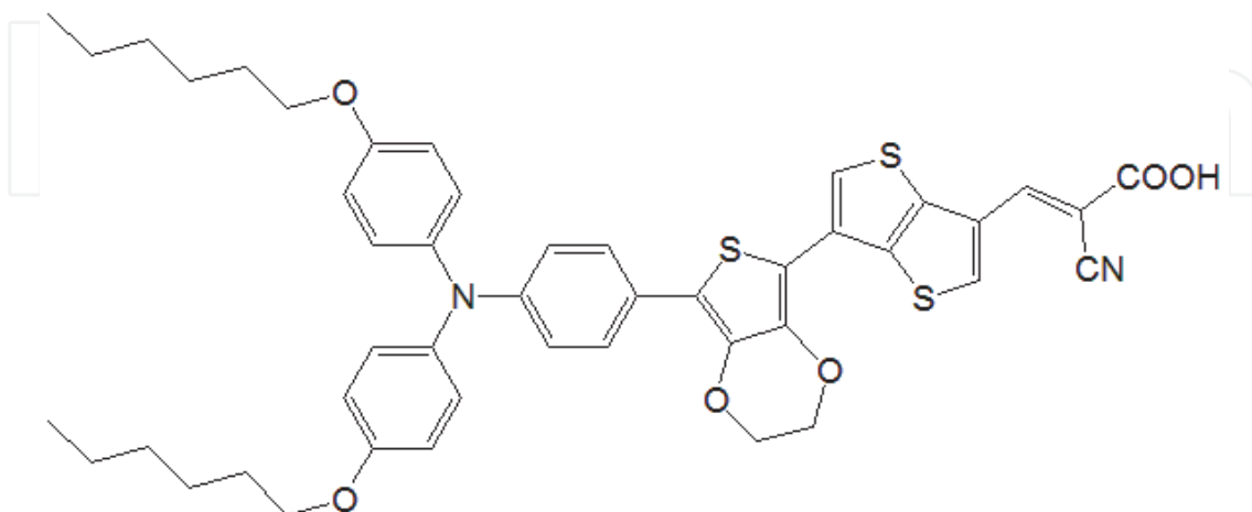
Fig. 38. C217 dye [35].
