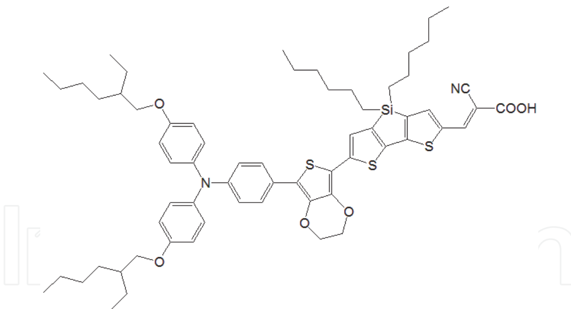
Fig. 39. C219 dye [36].
