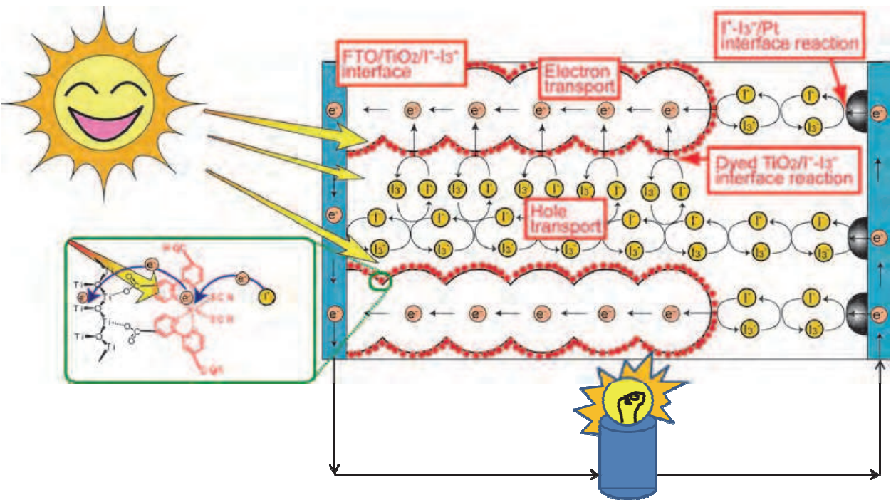
Fig. 5. Structure and electron movement in DSCs.
