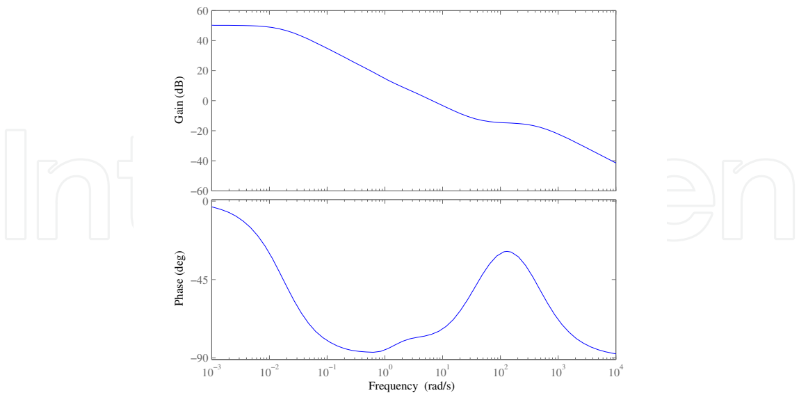
Fig. 15. Bode plot of the controller C(s)
