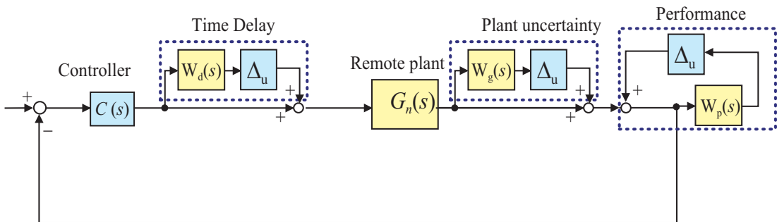
Fig. 16. Block diagram of the system with the conventinal controller
