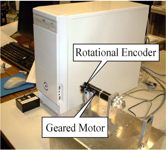
Fig. 13. Overview of the experimental device
