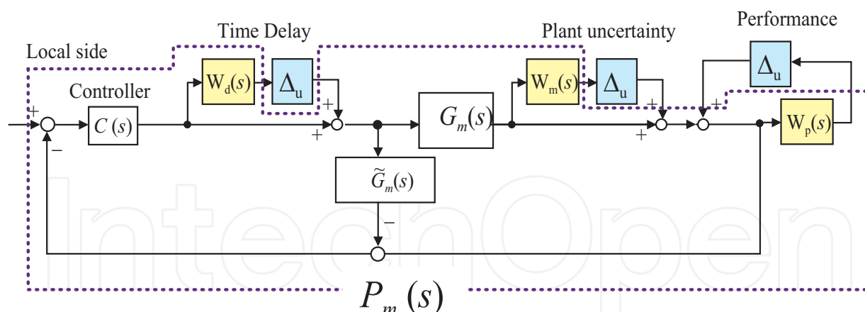
Fig. 10. Augmented plant P_m
