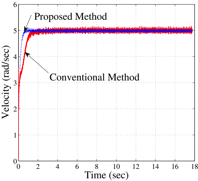
Fig. 17. Experimental results (Step response of velocity control)
