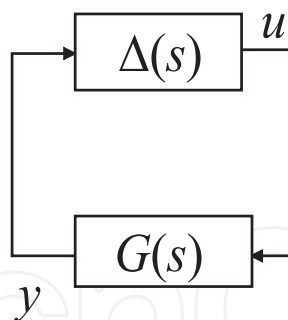
Fig. 1. Interconnection of a plant and time delay
