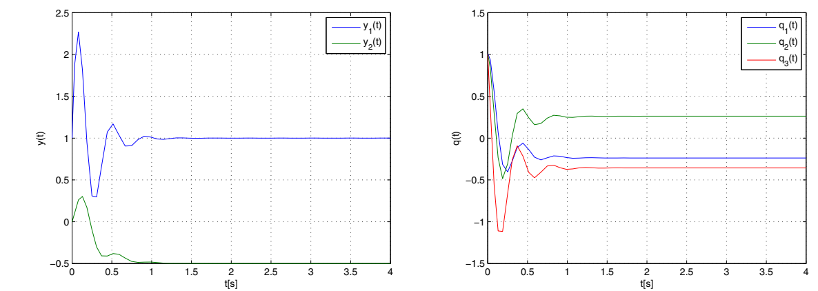
Fig. 3. System output and state response
