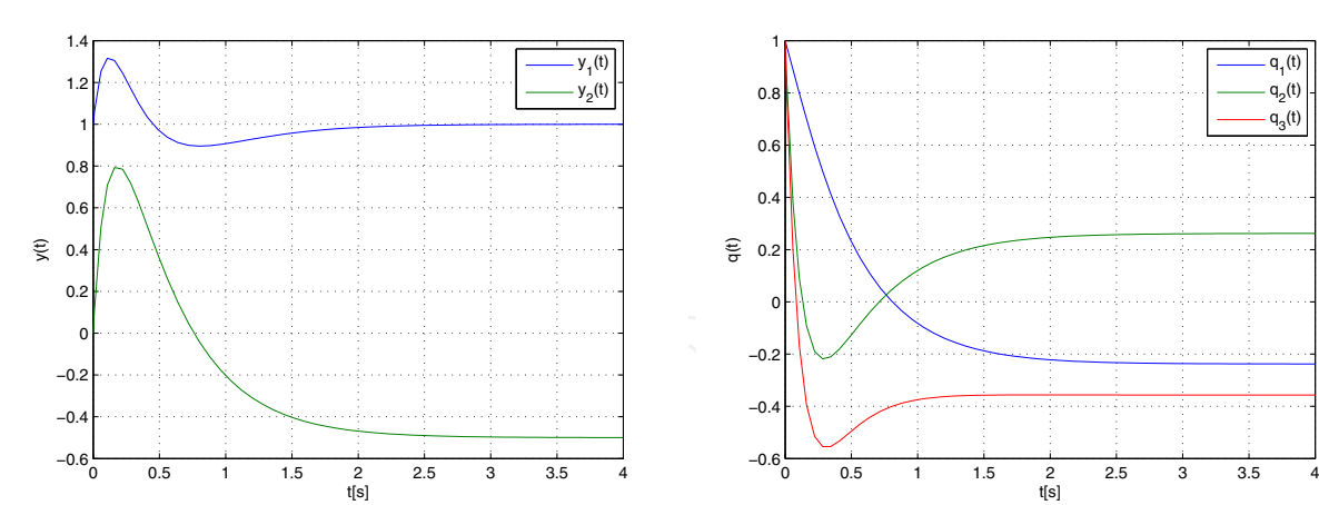
Fig. 2. System output and state response
