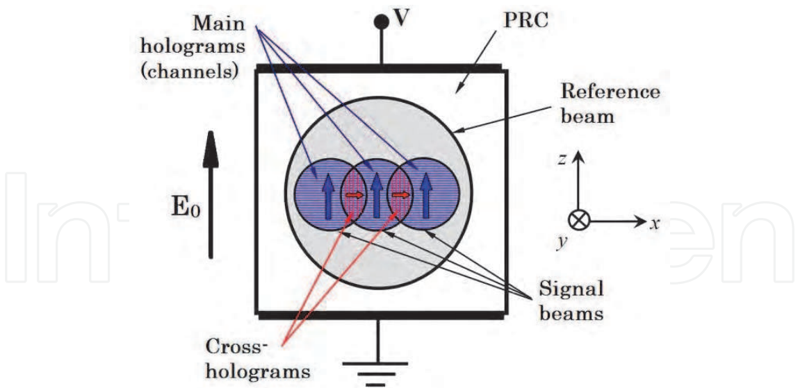
Fig. 10. Geometry of multi-wave mixing in PRC providing angular multiplexing of transmission dynamic holograms: all signal waves belong to horizontal plane ( xy ) and propagate in direction close to axis y ; the reference wave belongs to plane ( yz ) and makes the angle of 5^\circ with plane ( xy ) The normalized ultrasonic signals are shown in Fig. 11(b). From the measured signals it can be seen that the bulk longitudinal waves are clearly detected by all three channels with good sensitivity. The longitudinal wave arrives at different times at different sensor locations, providing information about the wave speed (related to material properties of the composite). The measured longitudinal velocity of 2480 m/s agrees well with data obtained for the same composite material by a different technique (Fomitchov, et al., 2001). Furthermore, the absence of any spurious signals in sensors 2 and 3 at the time of arrival of the ultrasonic wave packet at sensor 1 is an indication of the absence of cross-talk in the multichannel adaptive system based on dynamic holograms multiplexed in a PR crystal.
