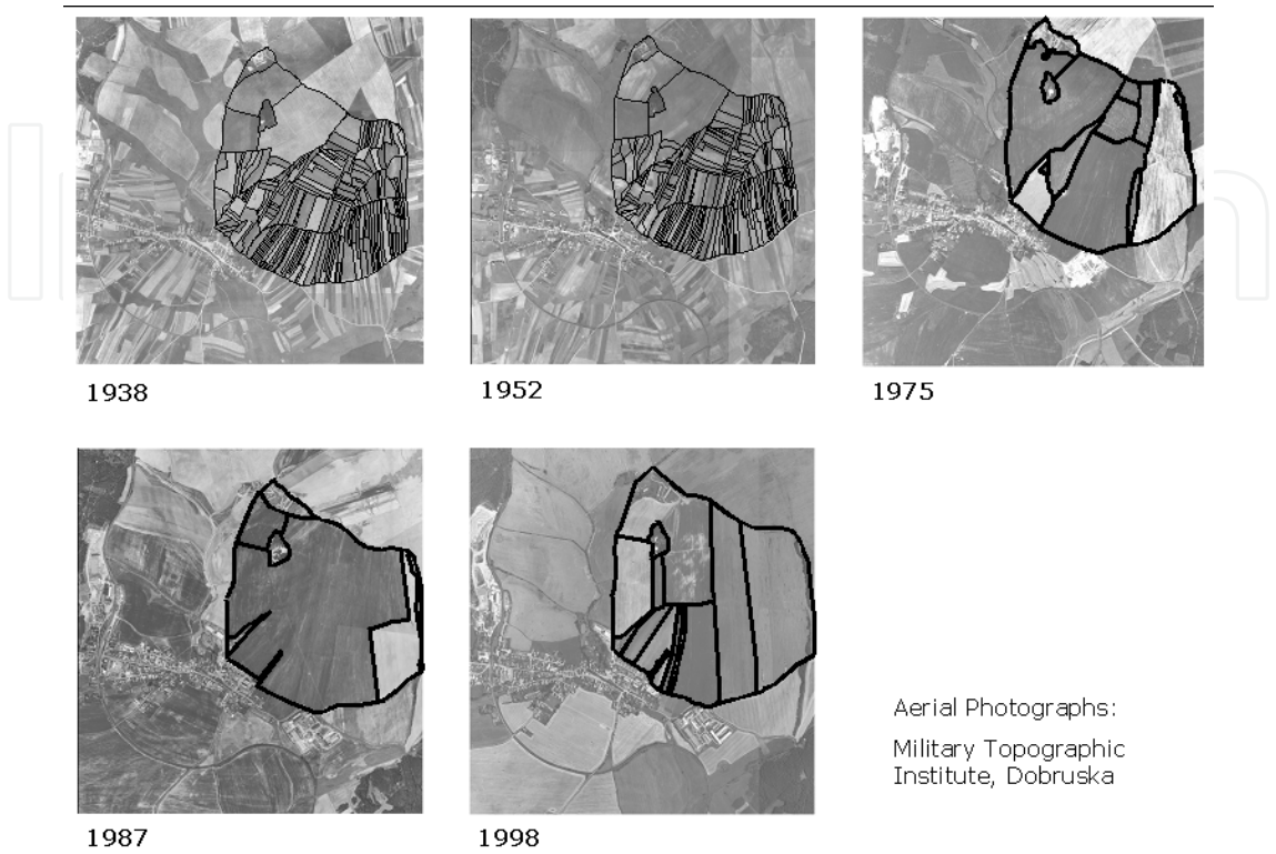
Fig. 5. Air images of a field about 1 km 2 in size, northeast of the town of Zihle in the basin of Lake Mladotice (see Fig. 2). Collective farming had the greatest impact between 1952 and 1975.
