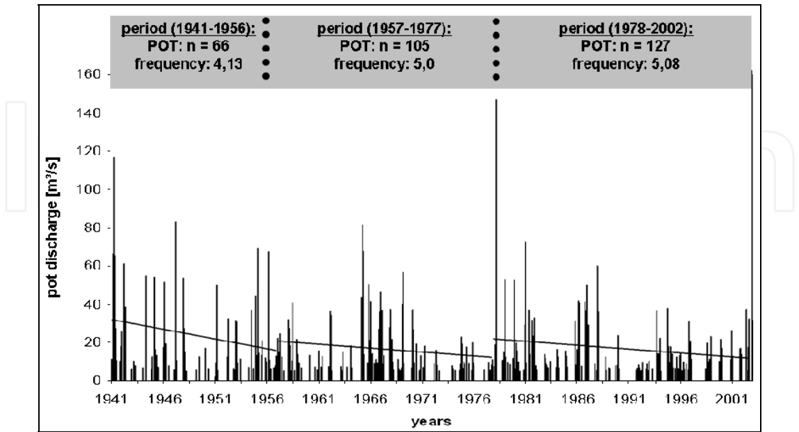
Fig. 6. Flood events at Plasy gauging station between 1941 and 2002, showing floods that exceed the threshold of 5.5 m 3 /s (pot = peaks over threshold).
