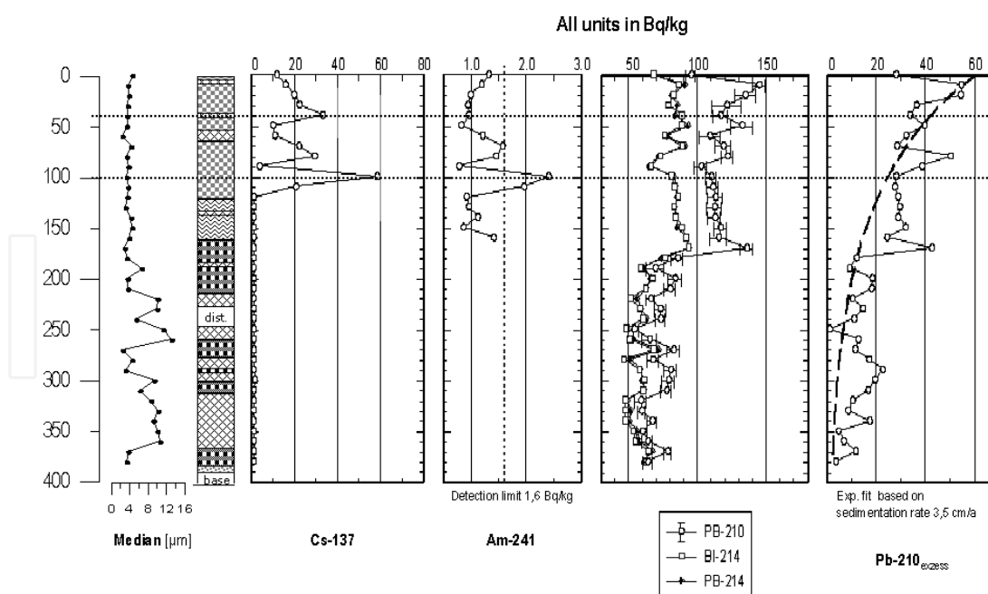
Fig. 9. Isotope contents in reference core ML 18/03 ( ^{137}\text{Cs} , ^{241}\text{Am} , ^{210}\text{Pb} ).
