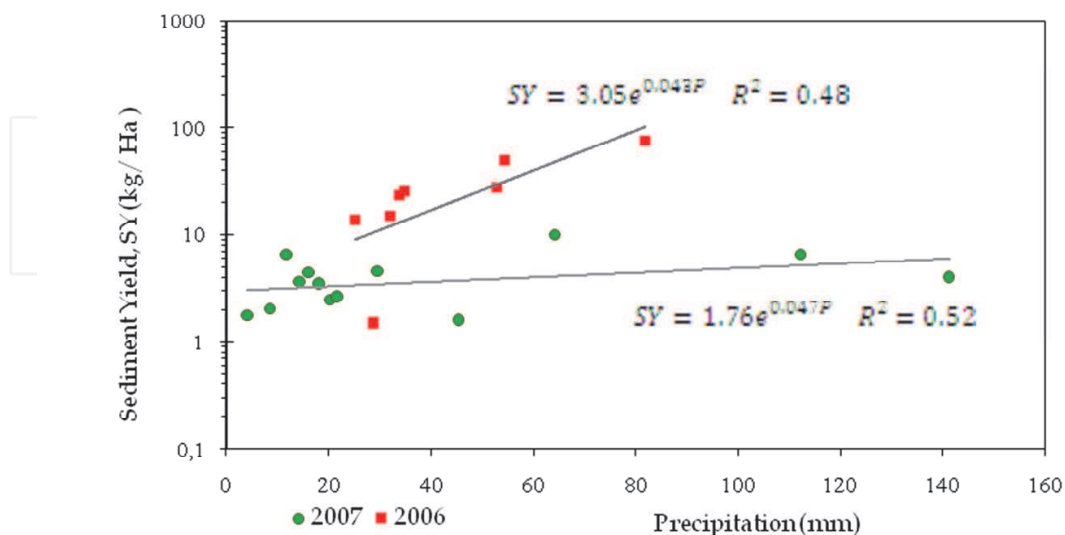
Fig. 5. Empirical relationships between sediment yield and precipitation height in 2006 and 2007.
