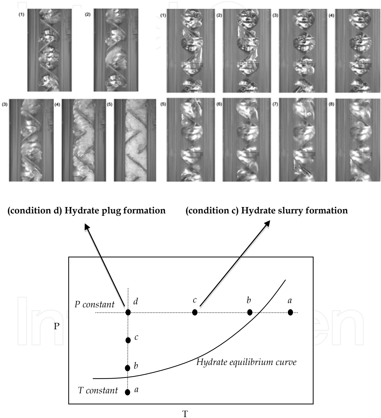
Fig. 4. Typical gas hydrate formation patterns in the semi-batch flow reactor. Conditions (a) and (b) are gas-water system, (c) and (d) are time-course in the hydrate formation, hydrate slurry and hydrate plug (Tajima et al., 2007)
