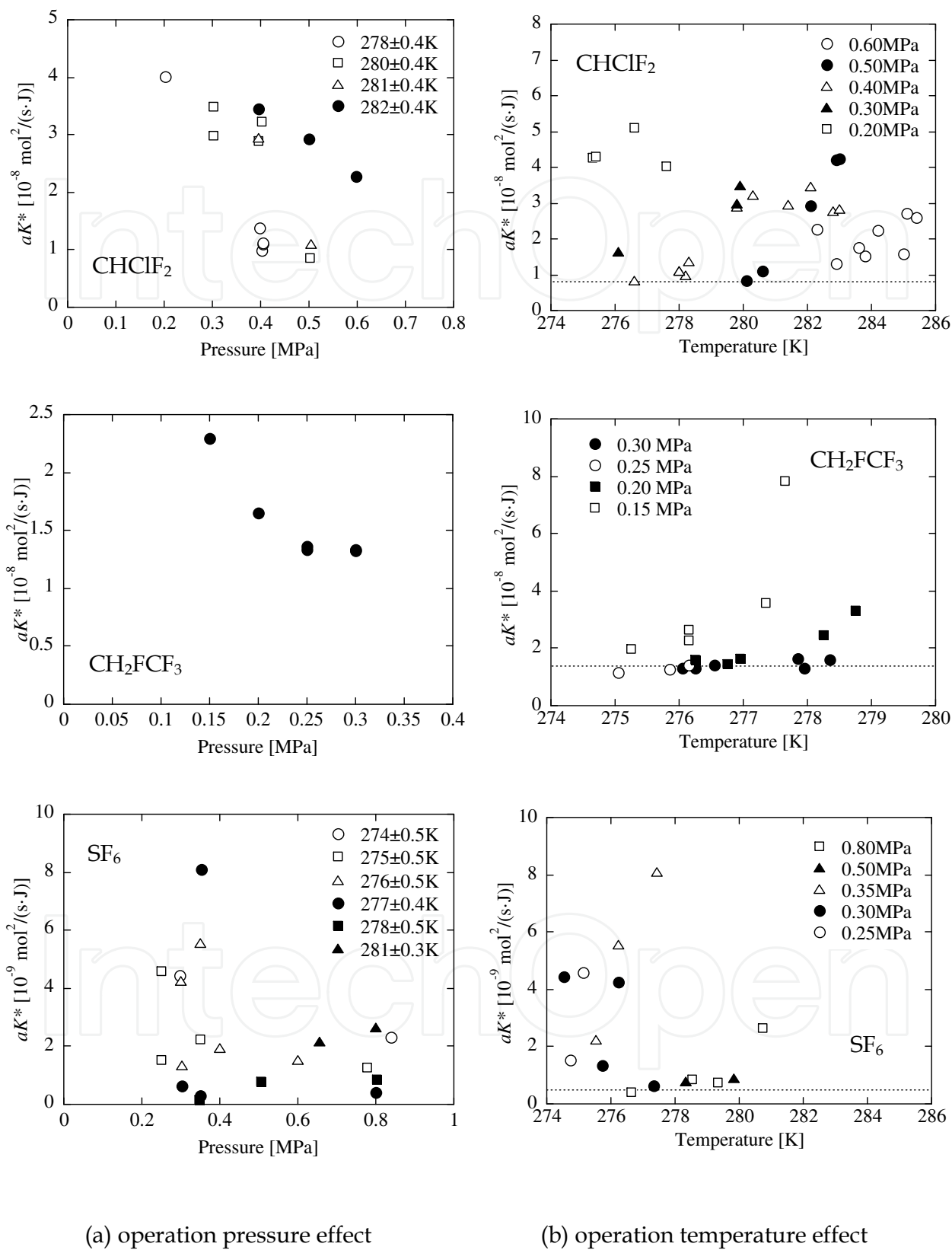
Fig. 5. Effect of operation pressure and temperature on the aK^* value of various gas hydrate at constant another one (Tajima et al., 2010a, 2011b).
