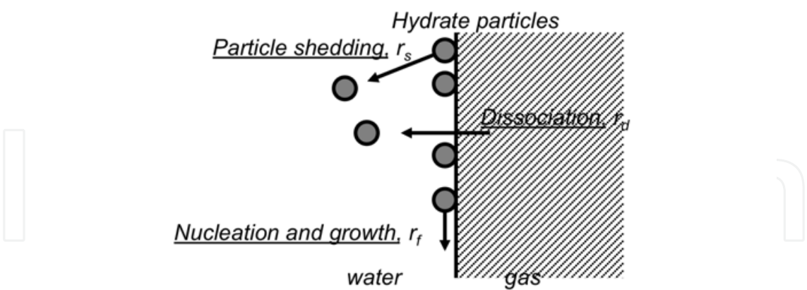
(a) Slurry formation, Higher r_d and r_s (large apparent interface area)
