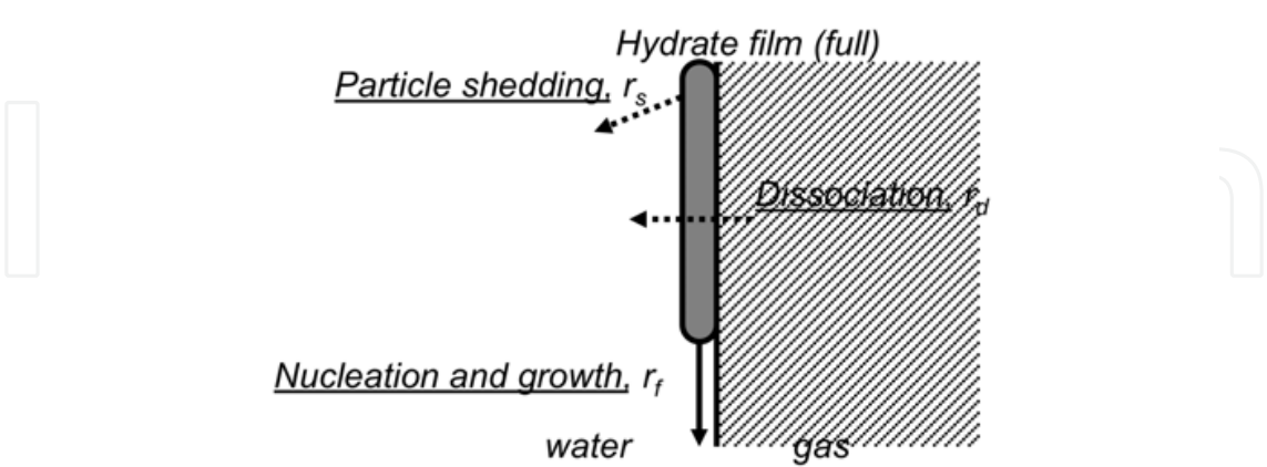
(c) Shell formation, Lower r_d and r_s (small apparent interface area)
