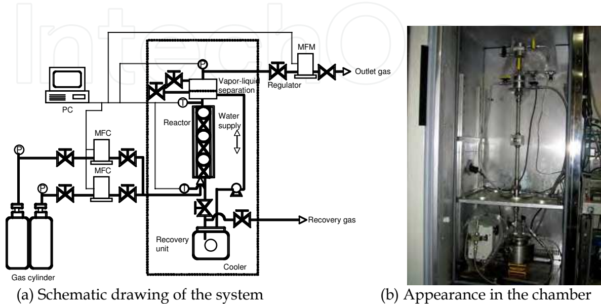
Fig. 1. Semi-batch flow reactor with static mixer for gas hydrate formation system
