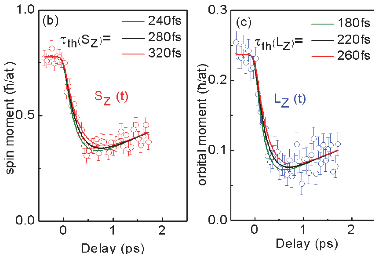
Fig. 7. Ultrafast dynamic of the spin and orbital magnetic moment measured using the pump probe set-up for a CoPd film at the CoL 2,3 edges. The X-ray probe beam are generated with the f-slicing set up at HZB-BESSY II leading to a time resolution of 130 fs [Boe2010]. Two different thermalization times were found for the spin and for the orbital magnetic moments. The best results of the fit procedure lead to \tau_{th}(S_Z) = 280 fs and \tau_{th}(L_Z) = 220 fs.
