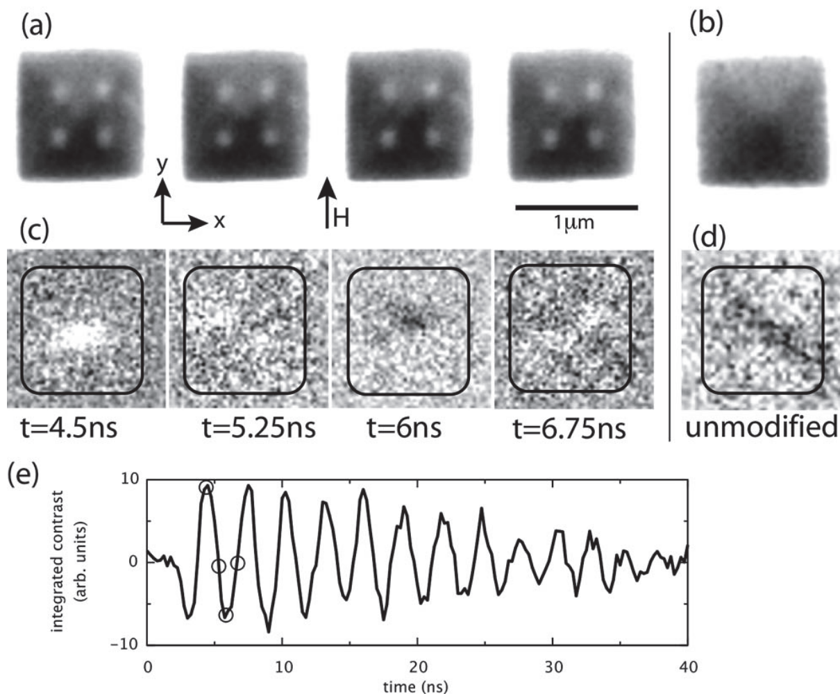
Fig. 2. (a) Sequence of STXM images for a 1\mu\text{m} \times 1\mu\text{m} \times 50\text{nm} modified square during one period of the oscillation. (b) image of an unmodified structure and shows that the domain wall motion can span a larger area of the structure when no defects are created. The intensity is proportional to the x component of the magnetization, revealing the Landau configuration and the small gyrotropic motion of the vortex structure. The total contrast in this sequence oscillates with the resonance frequency, as shown in (e). The four STXM images in (a) and (c) correspond to the four markers in (e). The magnetic pulse H starts at t=2\text{ns} . [Van 2008].
