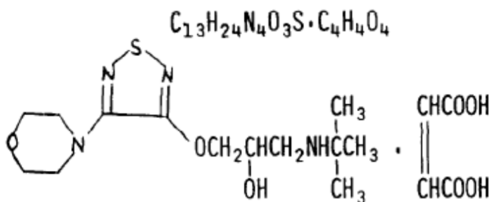
Fig. 1.0. Chemical structure and formula of timolol maleate
