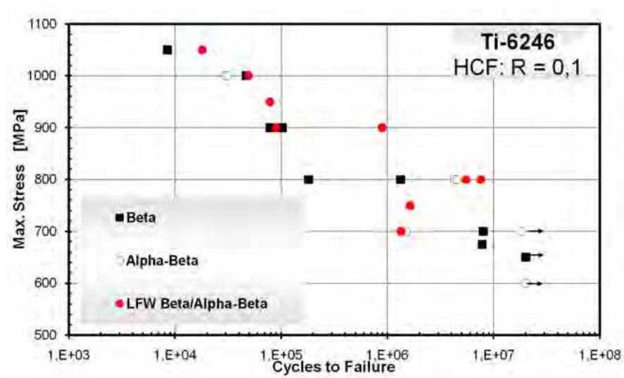
Fig. 20. HCF results for base materials and welds.
