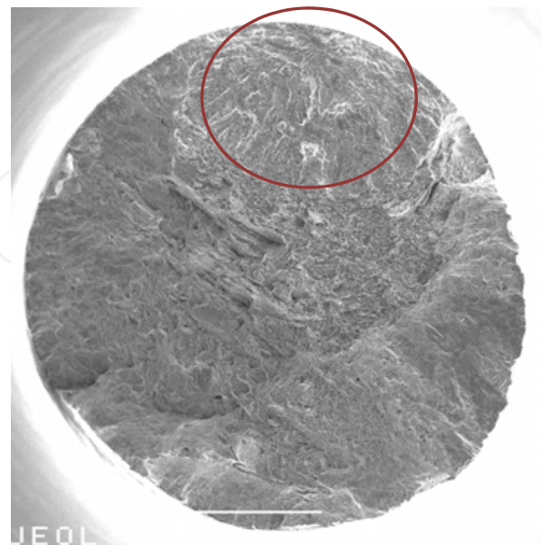
Fig. 21. Fracture surface of welded specimen tested at \sigma_{\max} = 800 MPa and failed after 6 \times 10^6 cycles. Circle indicates the origin of fatigue fracture.
