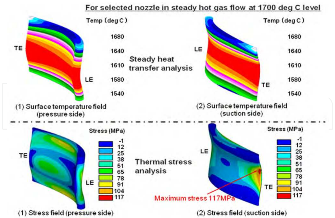
Fig. 17. Steady thermal stress generated during hot gas flow at 1700°C estimated by using numerical analysis.
