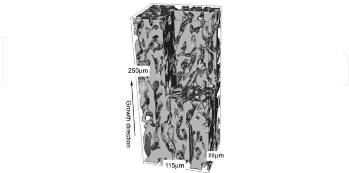
Fig. 4. Three-dimensional image of the unidirectionally solidified Al 2 O 3 /YAG eutectic structure. The \alpha -Al 2 O 3 phase was removed from image.
