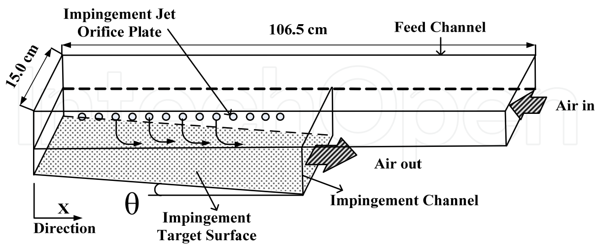
Fig. 7. Three-dimensional view of the test section
