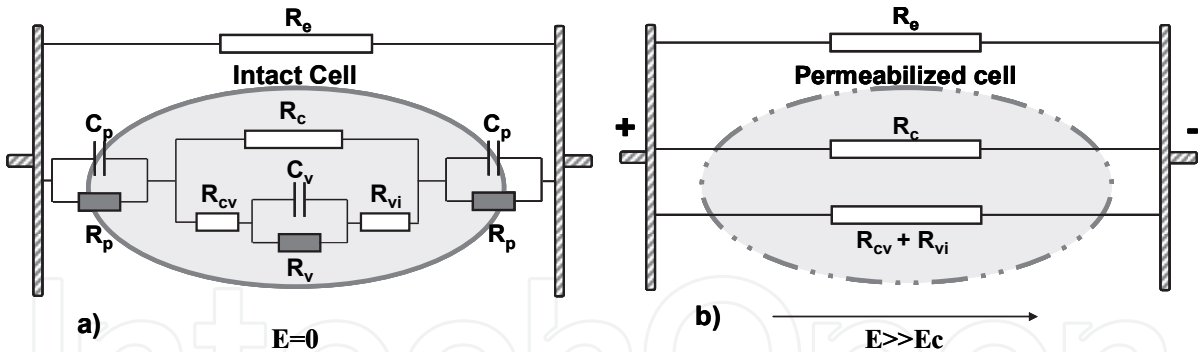
Fig. 3. Equivalent circuit model of (a) an intact and (b) ruptured plant cell. R_p, R_v , plasma and vacuole membrane (tonoplast) resistance; C_p, C_v , plasma and vacuole membrane (tonoplast) capacitance; R_c , cytoplasmic resistance surrounding the vacuole in the direction of current; R_{cv} , cytoplasmic resistance in vacuole direction; R_{vi} , resistance of the vacuole interior; R_e , resistance of the extracellular compartment (Adapted from Angersbach et al., 1999).
