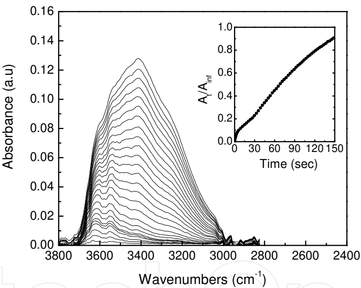
Fig. 8. Sequence of time-evolved spectra from PMMA sample treated at 25 °C.
