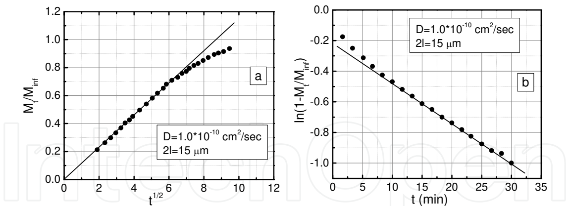
Fig. 2. Kinetics of mass uptake for a typical polymer. (a) M_t / M_\infty as function of t^{1/2} , (b) \ln(1 - M_t / M_\infty) as function of t ; data were extracted from literature (Fieldson and Barbari, 1993).
