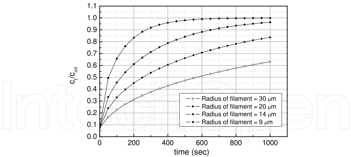
Fig. 3. C_t / C_\infty of dyeing versus t for different radius of fibers.
