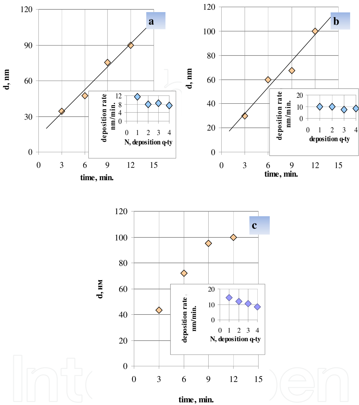
Fig. 2. The CdS thin film thickness dependence on time and quantity of deposition from aqueous solution: \text{CdCl}_2 (a); \text{CdSO}_4 (b); \text{CdI}_2 (c). The mean deposition rate of CdS thin films on figure inset.
