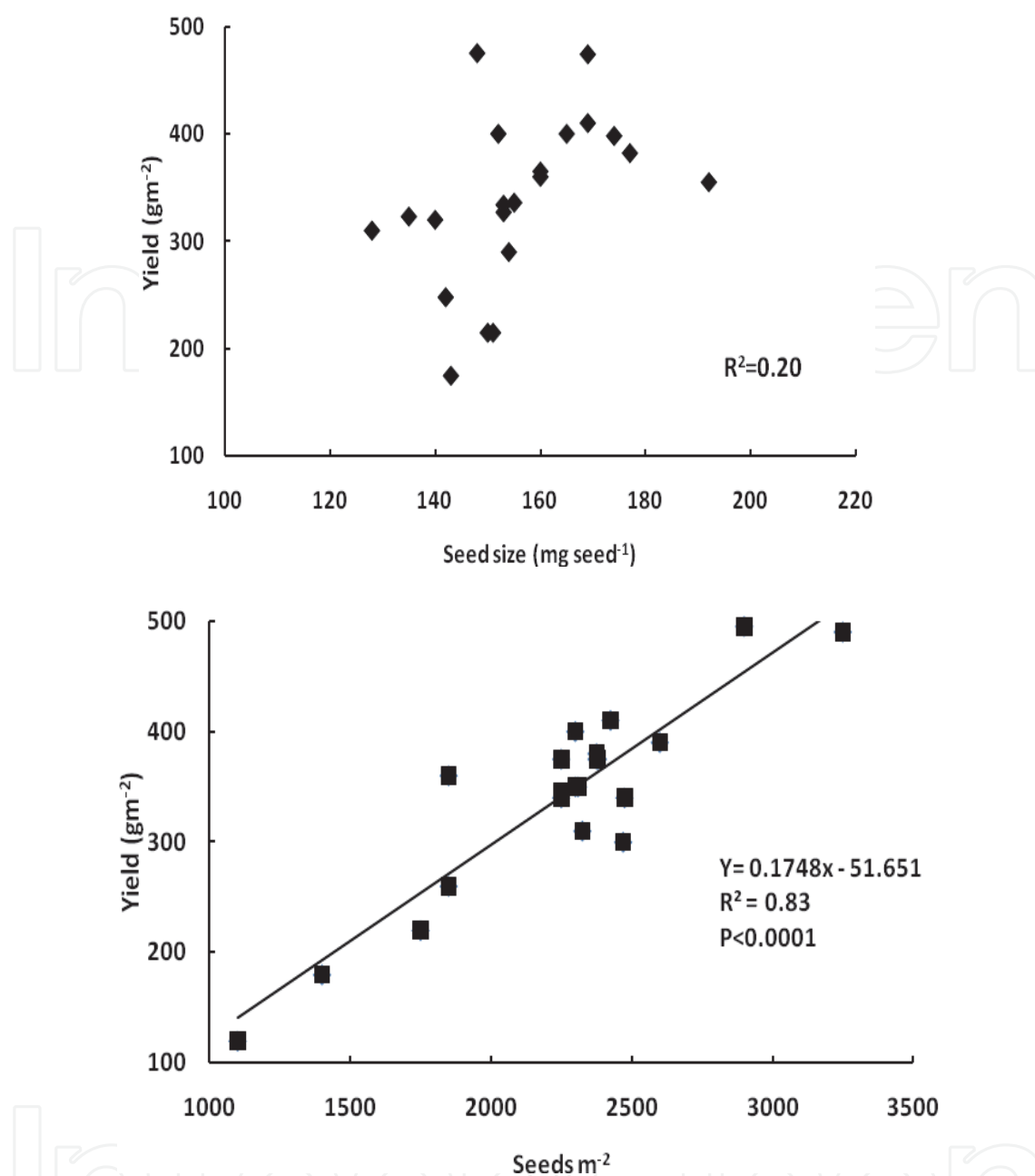
Fig. 5. The relationship of soybean yield with seed m -2 and seed size for cultivar Iroquois grown across 21 locations in the Midwestern US, 1996 (USDA, Unpublished data).
