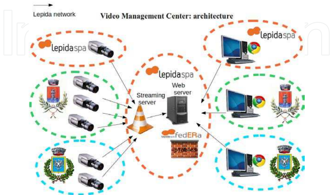
Fig. 13. Architecture for the management of camera strems produced by the Public Administrations.
