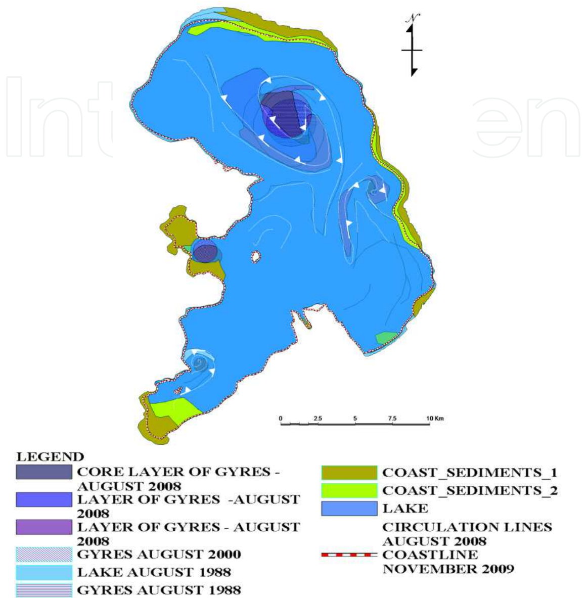
Fig. 14. Synthetic map concerning coastal sediment concentrations surface currents in the form of gyres.
