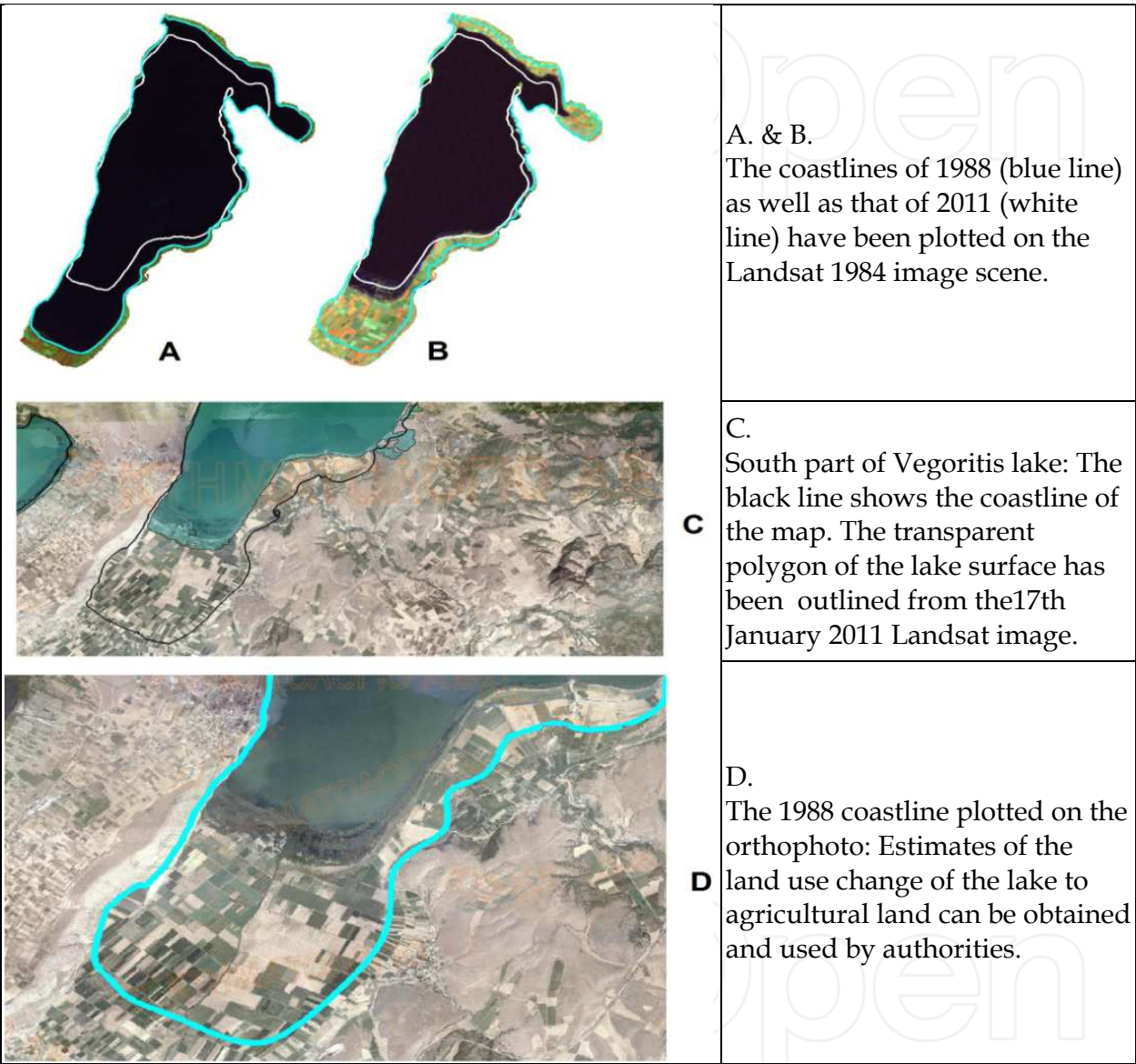
Fig. 10. Changes of the Vegorititis lake surface area.
