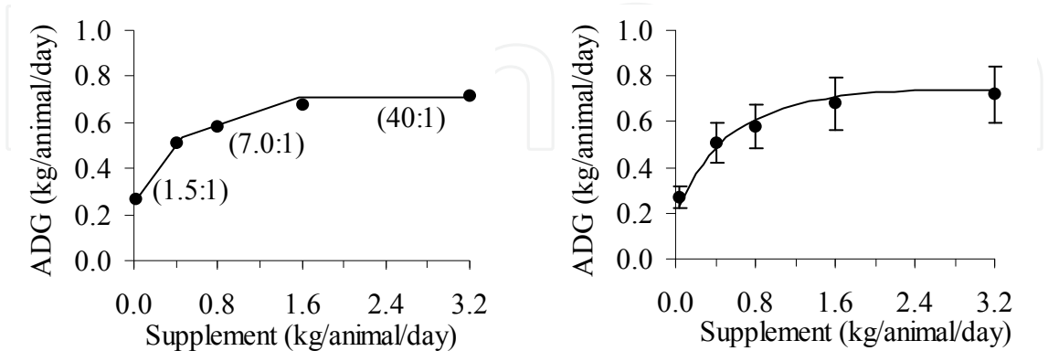
Fig. 6. Body weight gain (BWG) of growing bovines in pasture during the dry season, as a function of daily intake of supplement with 24% CP, in which the values among parenthesis represent the differential in kilograms of supplement given daily divided by the differential in weight gain, in relation to the previous treatment (Lana, 2005; Lana et al., 2005)
