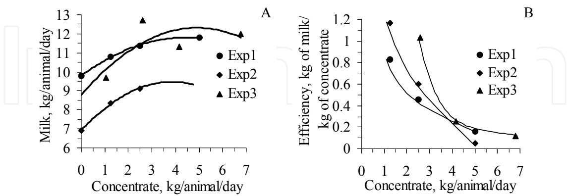
Fig. 7. Production of milk (A) and efficiency of use of concentrate (B) as a function of intake of increasing level of concentrate in three experiments (Pimentel et al., 2006b, 2006c; Teixeira et al., 2006)
