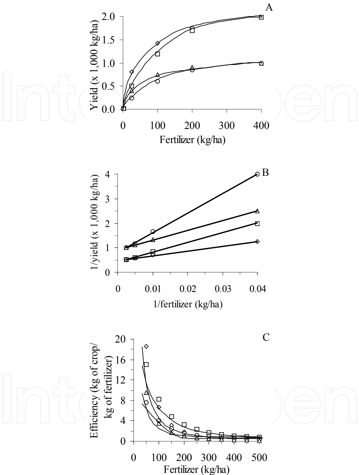
Fig. 4. Biological responses to nutrients as a function of a second limiting nutrient (A) - control (O), decrease in k_s ( \Delta ), increase in k_{max} ( \square ) and decrease in k_s and increase in k_{max} ( \diamond ); reciprocal of production as a function of reciprocal of fertilizer level - plot of Lineweaver-Burk (B); and effect of a second limiting nutrient in the efficiency of use of the first one (C)
