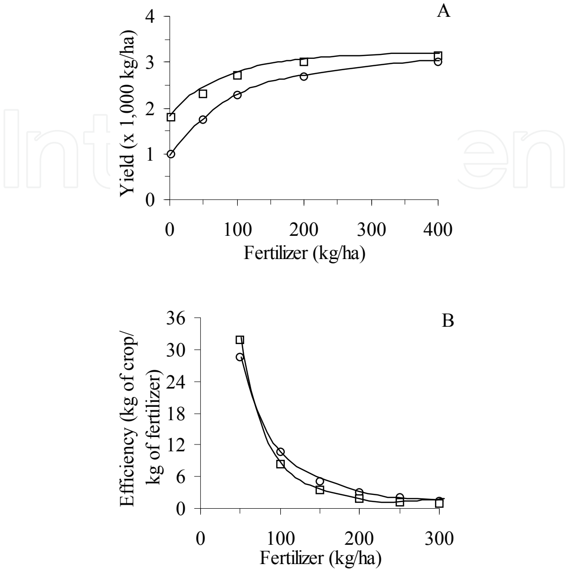
Fig. 5. Plants responses to fertilizers in low (O) and high (□) soil fertility (A); and the effect of soil fertility in the efficiency of use of fertilizer (B)
