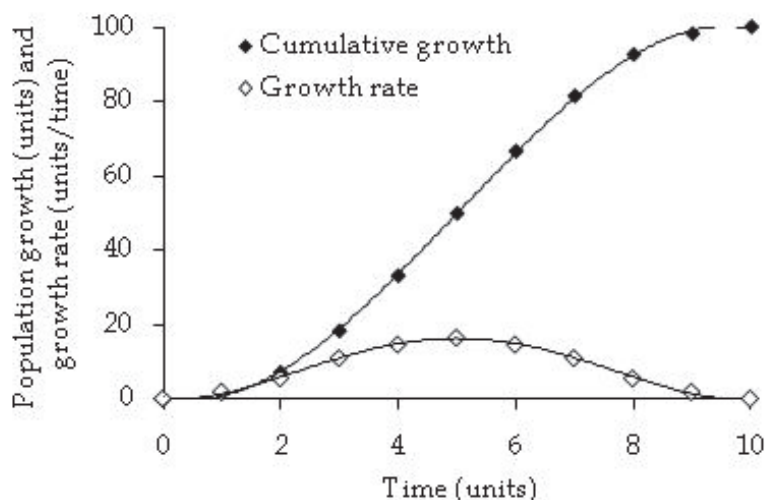
Fig. 3. Theoretical population growth (cumulative and growth rate) as function of time.
