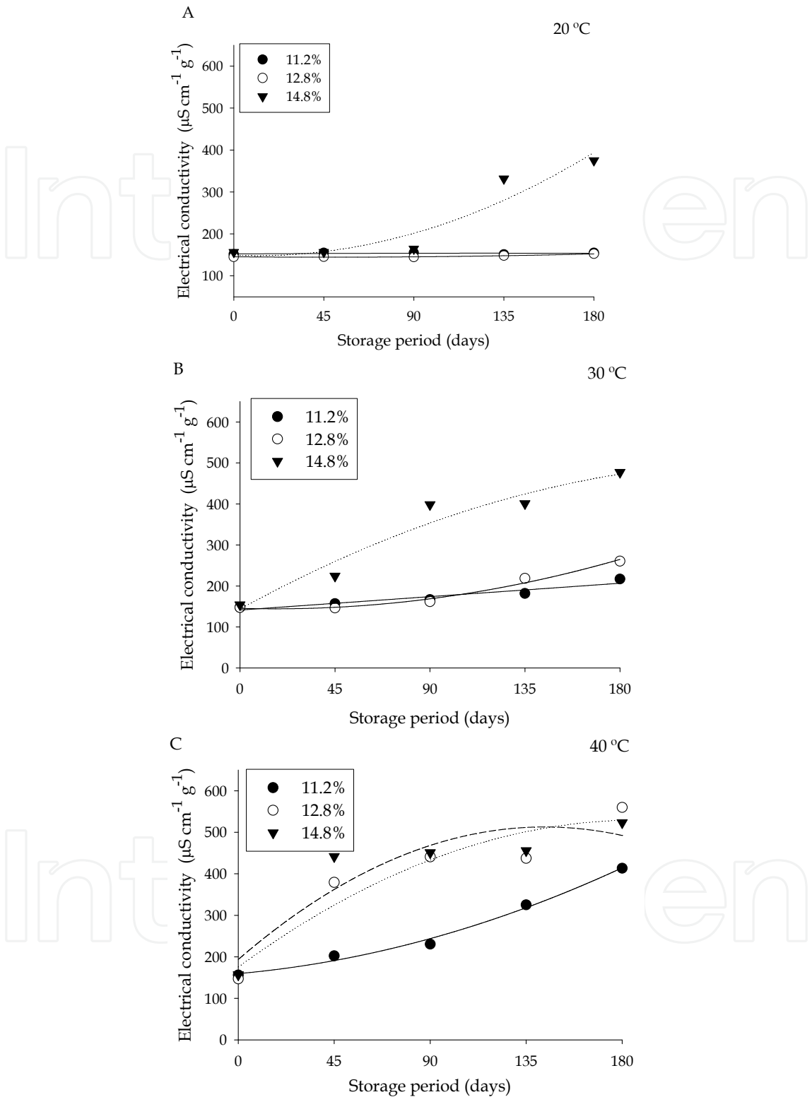
Fig. 3. Regression curves of electrical conductivity ( \mu\text{S cm}^{-1} \text{g}^{-1} ) of the solution which contains soybeans stored with moisture contents of 11.2, 12.8 and 14.8% w.b. at the temperatures of 20, 30 and 40 °C.
