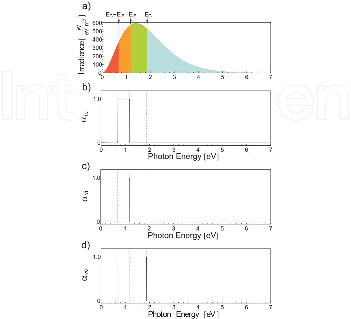
Fig. 4. (a) Radiant emittance of a blackbody at a temperature of 5760 K. Below, plots of the absorption coefficients for (b) IB→CB, (c) VB→IB and (d) VB→CB transitions. The shape of these functions depends on the energy gap and the assumptions made. The depicted forms allow to determine the integral boundaries in equations (12), (13) and (14).
