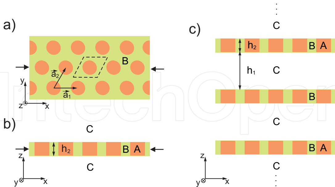
Fig. 9. Structure of a periodic slab with inclusions in triangular lattice, (a) top and (b) side view. Letters A, B and C denote the inclusion, matrix and spacer materials, respectively. The arrows indicate the cross-section plane. Dashed parallelogram in (a) delimits the unit cell, which reproduces the whole plane when translated by superlattice vectors \mathbf{a}_1 and \mathbf{a}_2 . (c) The supercell structure used in the plane wave method: an infinite stack of replicas of the periodic slab.
