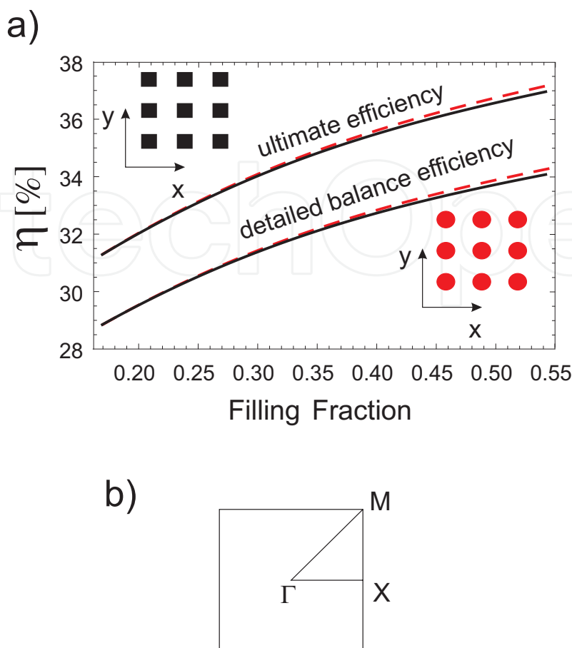
Fig. 11. (a) Detailed balance efficiency and ultimate efficiency of solar energy conversion versus filling fraction for a slab (of thickness h_2=50\text{\AA} ) with cylinders (dashed red line) and square prisms (solid black line) arranged in a square lattice (the lattice constant of the superlattice is a = 50\text{\AA} ). The inclusion, slab and spacer materials are GaAs, \text{Al}_{0.35}\text{Ga}_{0.65}\text{As} and AlAs, respectively. (b) The high-symmetry line in the first Brillouin zone used in the search of absolute minigaps.
