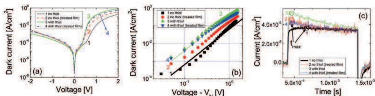
Fig. 17. The improvement in charge carrier mobility in treated (annealed films and films fabricated with processing additive) compared to pristine films demonstrated by two methods: dark current-voltage injection and CELIV. (a) log-lin plot showing the rectification ratio in forward and reverse bias and insignificant differences in leakage current in reverse bias. (b) log-log plot in forward bias showing much higher injection current levels in treated blends. (c) faster carrier extraction in treated films compared to pristine directly measured by CELIV current transients. Improvement in the carrier mobility can be seen from the shift in the position of extraction maximum, while experimental conditions (film thicknesses and applied voltages) were kept similar. Thermal annealing of films fabricated with processing additive results in no change in performance. Reprinted with permission from (Pivrikas et al., 2008). Copyright 2008, with permission from Elsevier.
