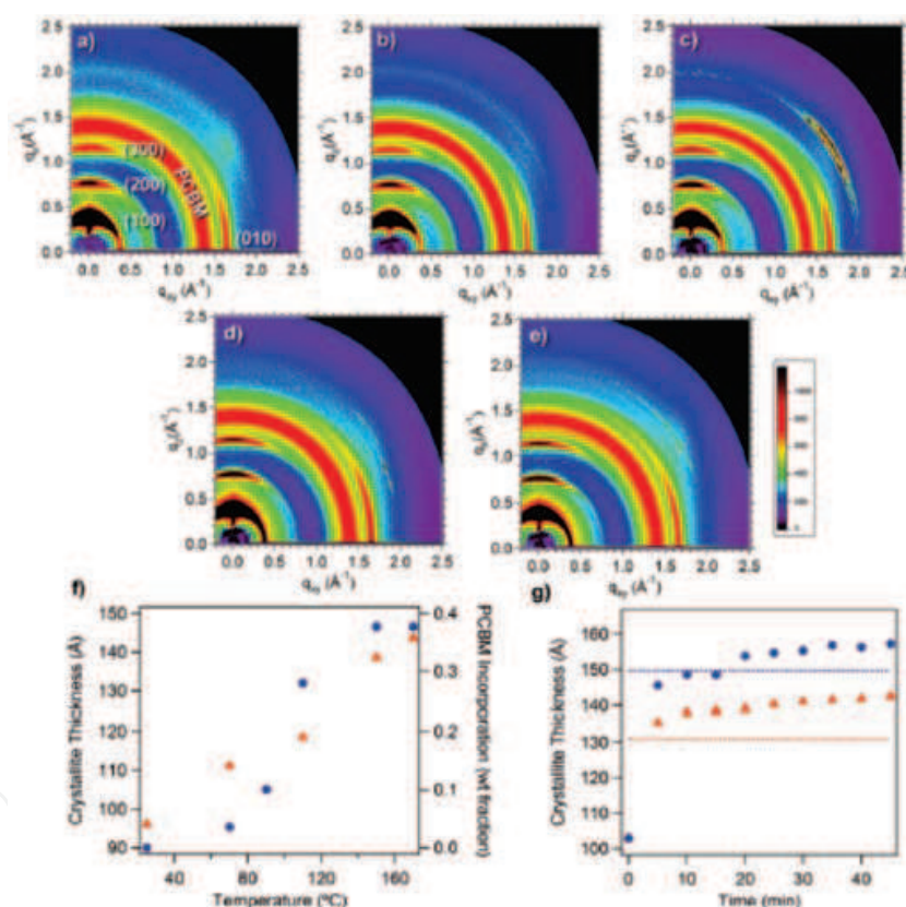
Fig. 7. Two-dimensional GIWAXS of a P3HT/PCBM bilayer on Si a) as-cast and annealed at b) 70 °C, c) 110 °C, d) 150 °C, and e) 170 °C for 5 min. f) The Scherrer equation was used to extract the P3HT crystallite thickness along the a -axis from the full-width-at-half-maximum of the (100) reflection. PCBM incorporation from the DSIMS measurements was plotted for comparison at various annealing temperatures. g) Growth in the crystal thickness with time using in-situ heating 2D GIWAXS of a P3HT/PCBM bilayer on Si at 110 °C (orange) and 170 °C (blue). The Scherrer equation was used to determine crystal thickness from the (100) reflection corresponding to P3HT. The dotted line corresponds to a neat P3HT/Si sample heated for 5 min at 110 °C (orange) and 170 °C (blue). Copyright 2011 Wiley. Used with permission from (Treat et al., 2011).
