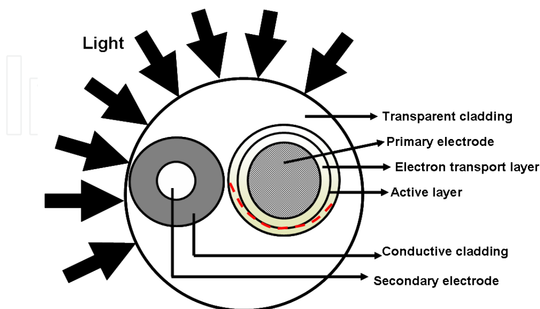
Fig. 3. Photovoltaic fibre
