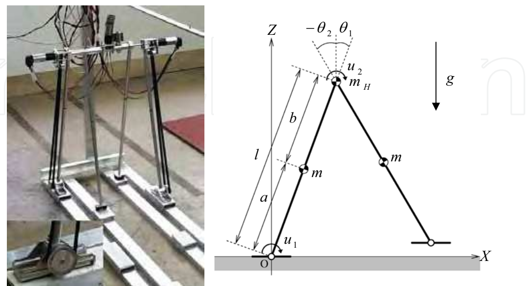
Fig. 1. Experimental walking machine and its foot mechanism (left), and its ideal model (right).
