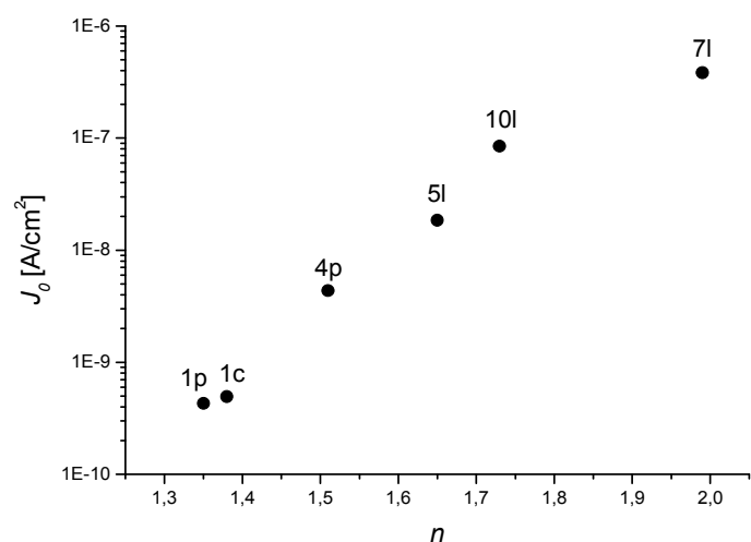
Fig. 9. Saturation current density dependence on ideality factor (Vasic et al., 2000).
