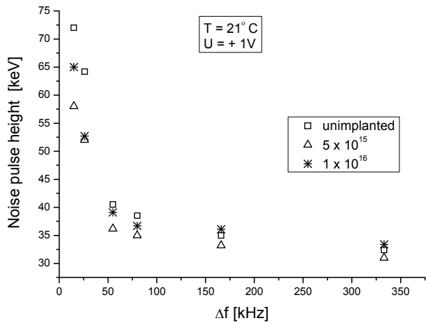
Fig. 2. Frequency noise level for TiN/Ti/Si samples at 21°C (Vasic et al., 2011).
