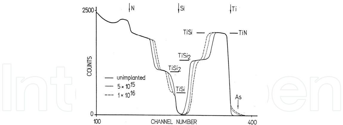
Fig. 1. RBS spectra of TiN/Ti/Si samples (Vasic et al., 2011).
