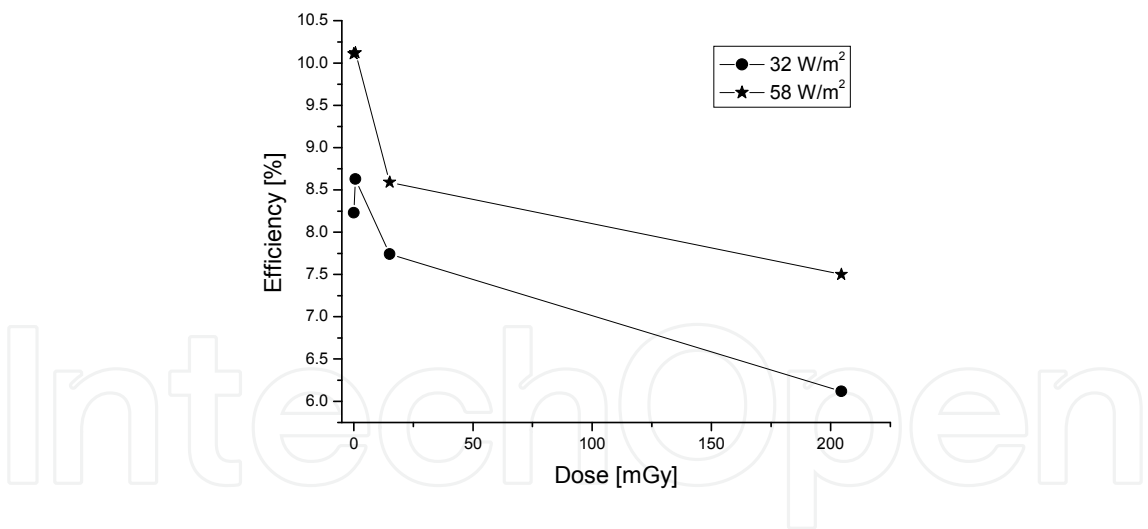
Fig. 15. Dependence of the efficiency on doses (Vasic et al., 2008).
