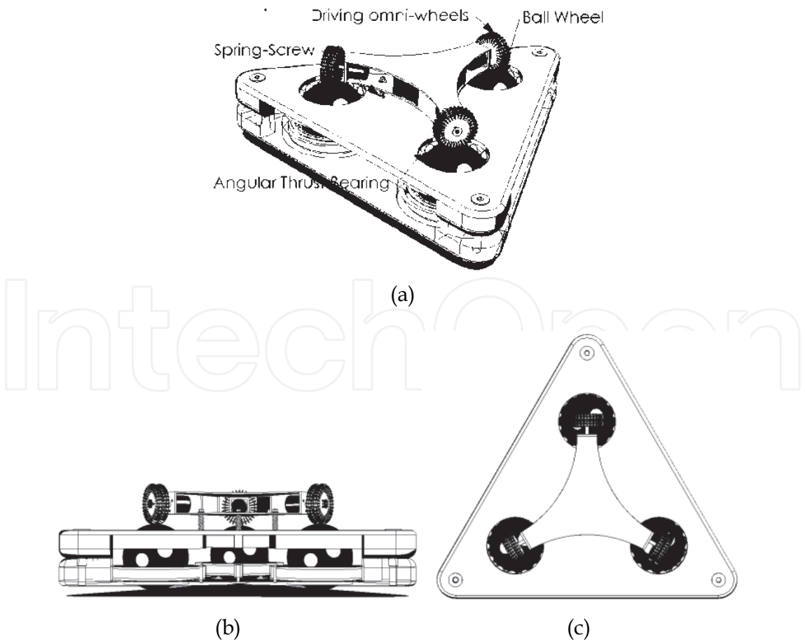
Fig. 1. First type Spherical wheel robot, a) Isometric View, b) Side View, c) Top View
