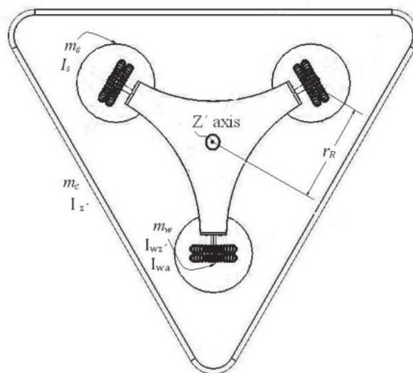
Fig. 7. Robot mass and inertia properties
