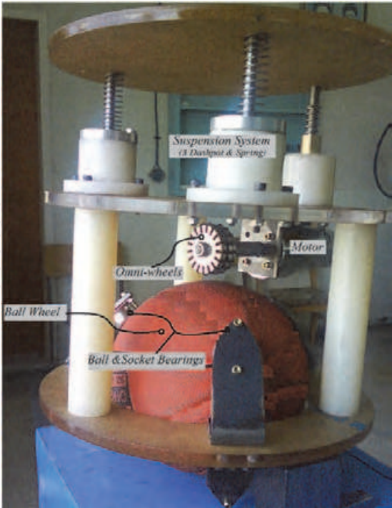
Fig. 3. BWR-2 modular driving system A list of robot geometric and physical parameters is summarized in Table 1.
