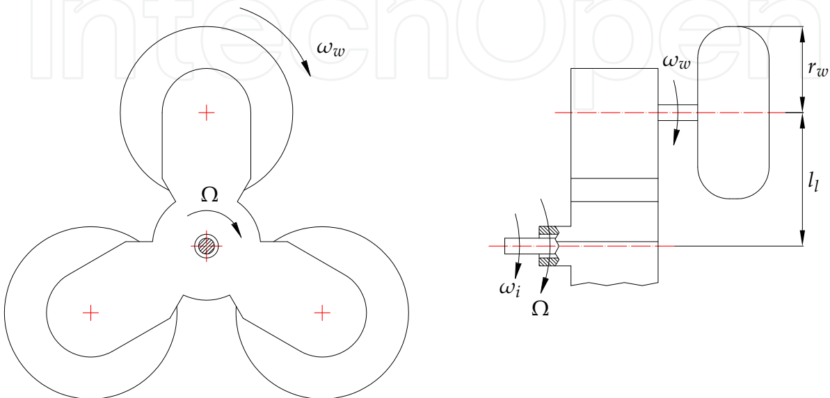
Fig. 5. Driving unit scheme
