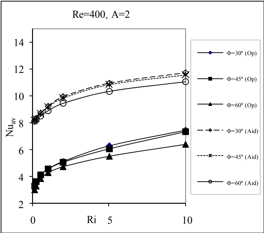
Fig. 17. Variation of Nu_{av} with Ri at A=2 , Re=400
