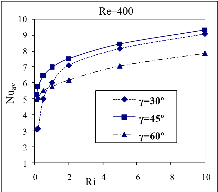
Fig. 8. Average Nusselt number, Nu_{av} vs Richardson number at Re=400 , A=1
