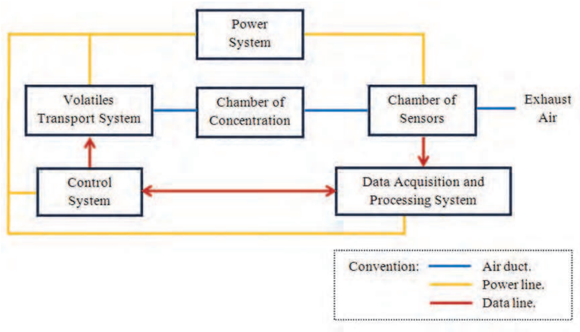
Fig. 4. Block diagram representing the electronic nose system.
