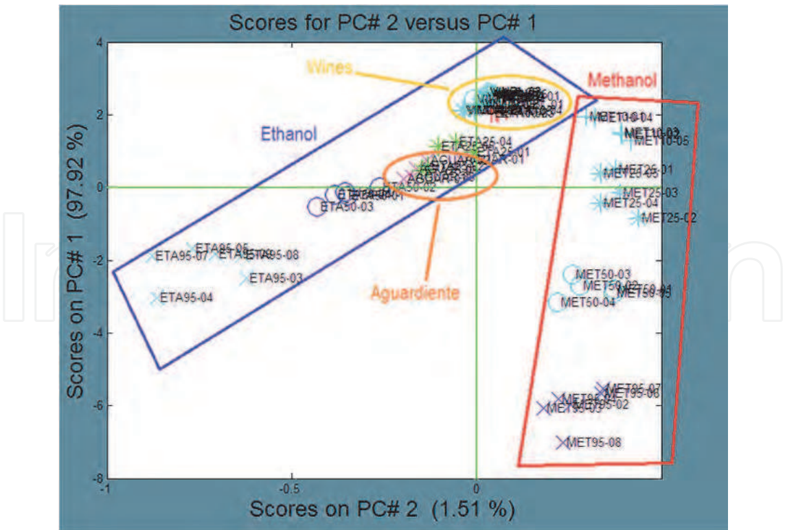
Fig. 14. Results of PCA analysis for the classification of wines and Aguardiente, according to the concentration of Ethanol and Methanol.
